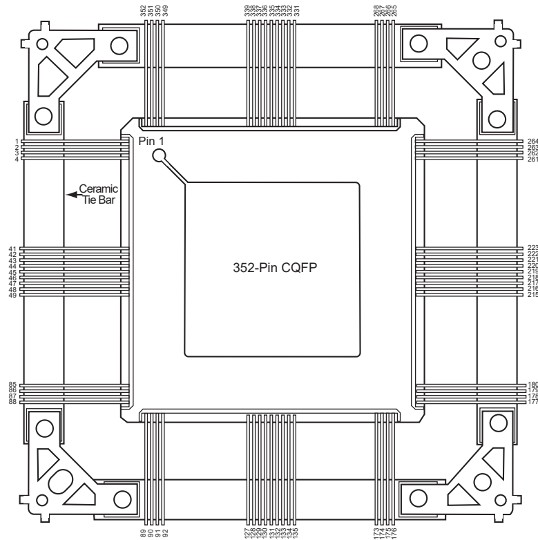
Figure 3-11. Package Bottom-View
