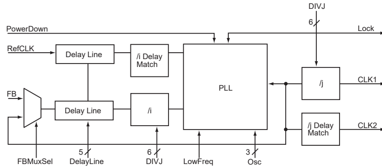
Figure 2-49. PLL Block Diagram
