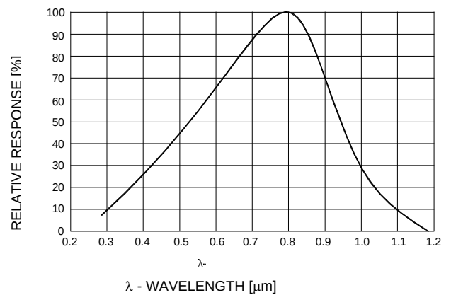
RELATIVE SPECTRAL RESPONSE
