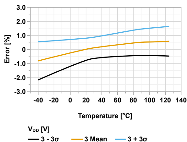
Figure 51-88. CDAFVR Voltage Error vs. Temperature ( V_{DD} = 3.0V , V_{REF} = 2.048V )
