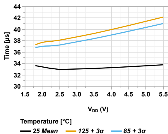
Figure 51-36. Wake-up Time (COSC[2:0] = 'b110, OSCFRQ = 16 MHz, VREGPM[1:0] = 'b01 = LP) vs. V_{DD}
