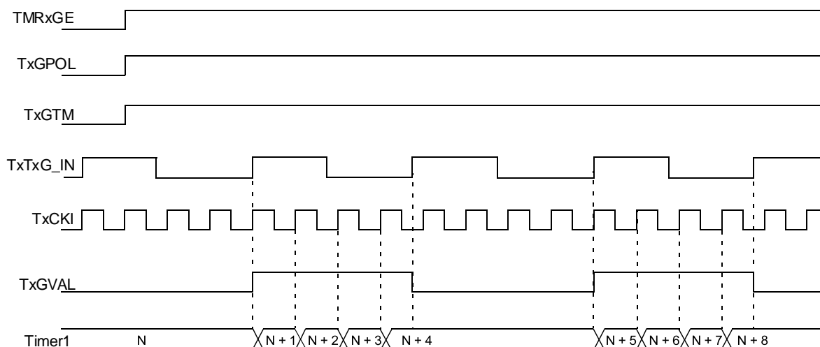
Figure 27-5. Timer1 Gate Toggle Mode
