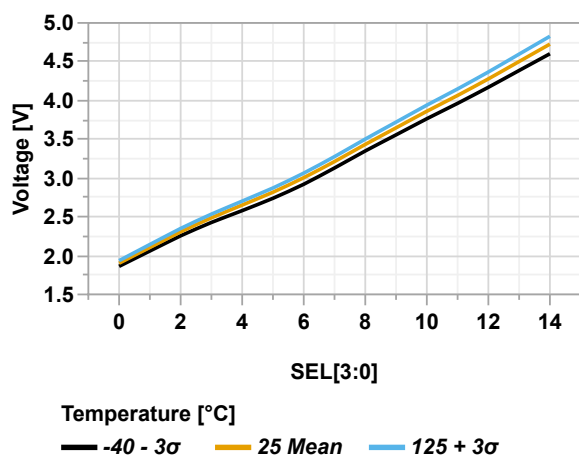
Figure 51-56. HLVD Negative Edge SEL[3:0] vs. Temperature
