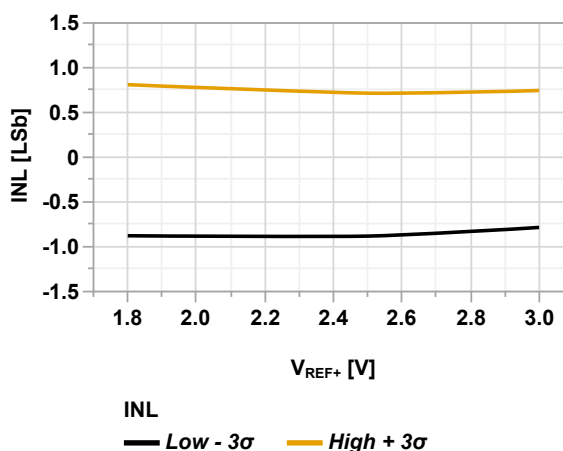
Figure 51-112. INL vs. V_{REF+} (ADC Differential Mode, T_{AD} = 1 \mu s , V_{DD} = 3.0V , T = 125^\circ C , CPON = 1 )
