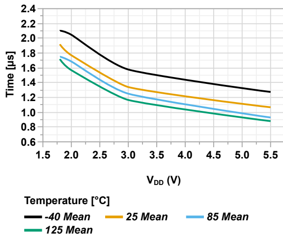
Figure 51-176. Turn-On Time Over V_{DD} and Temperature
