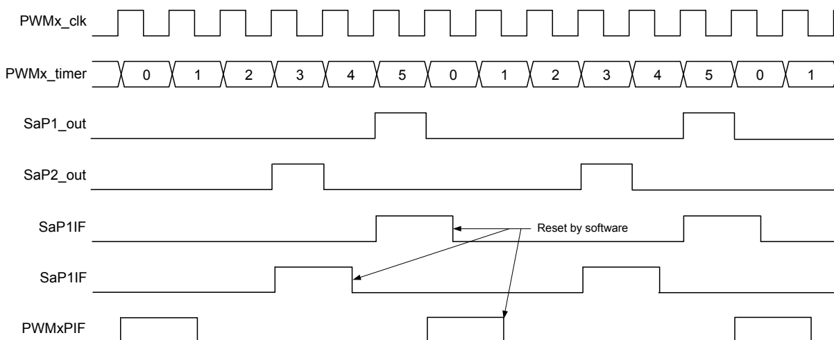
Figure 32-10. Pulsed Compare Timing Diagram
