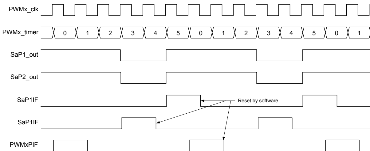
Figure 32-8. Variable Alignment Timing Diagram
