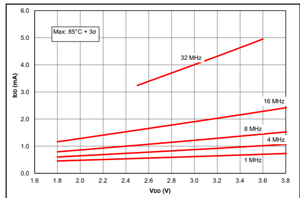
FIGURE 36-6: I_{DD} Maximum, HFINTOSC Mode, PIC16LF1614/8 Only.
