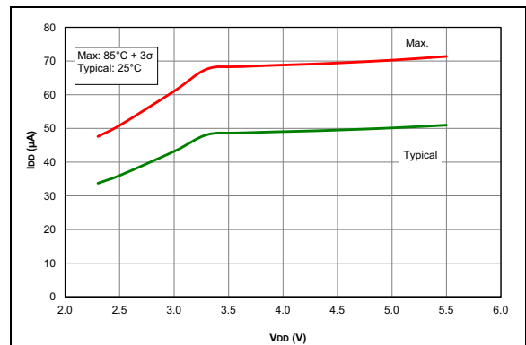
FIGURE 36-12: I_{DD} , EC Oscillator LP Mode, F_{OSC} = 500\text{ kHz} , PIC16F1614/8 Only.
