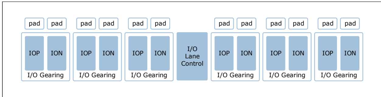
Figure 4-4. I/O Topology
