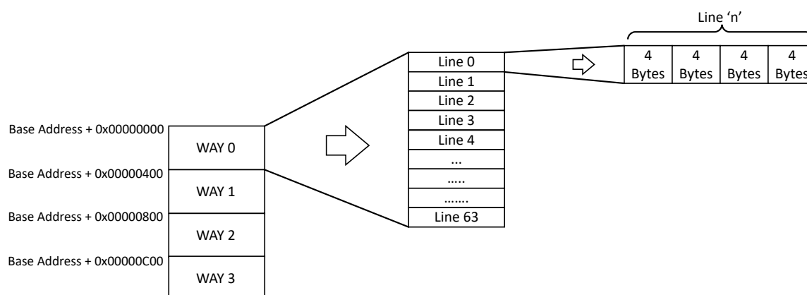
Figure 11-2. CMCC Organization
