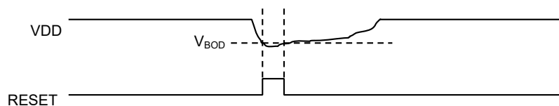
Figure 56-2. BOD33 Hysteresis OFF
