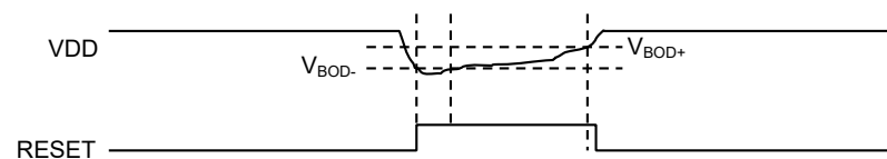
Figure 56-3. BOD33 Hysteresis ON
