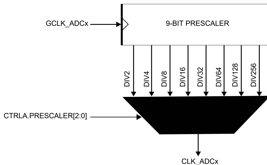
Figure 45-2. ADC Prescaler
