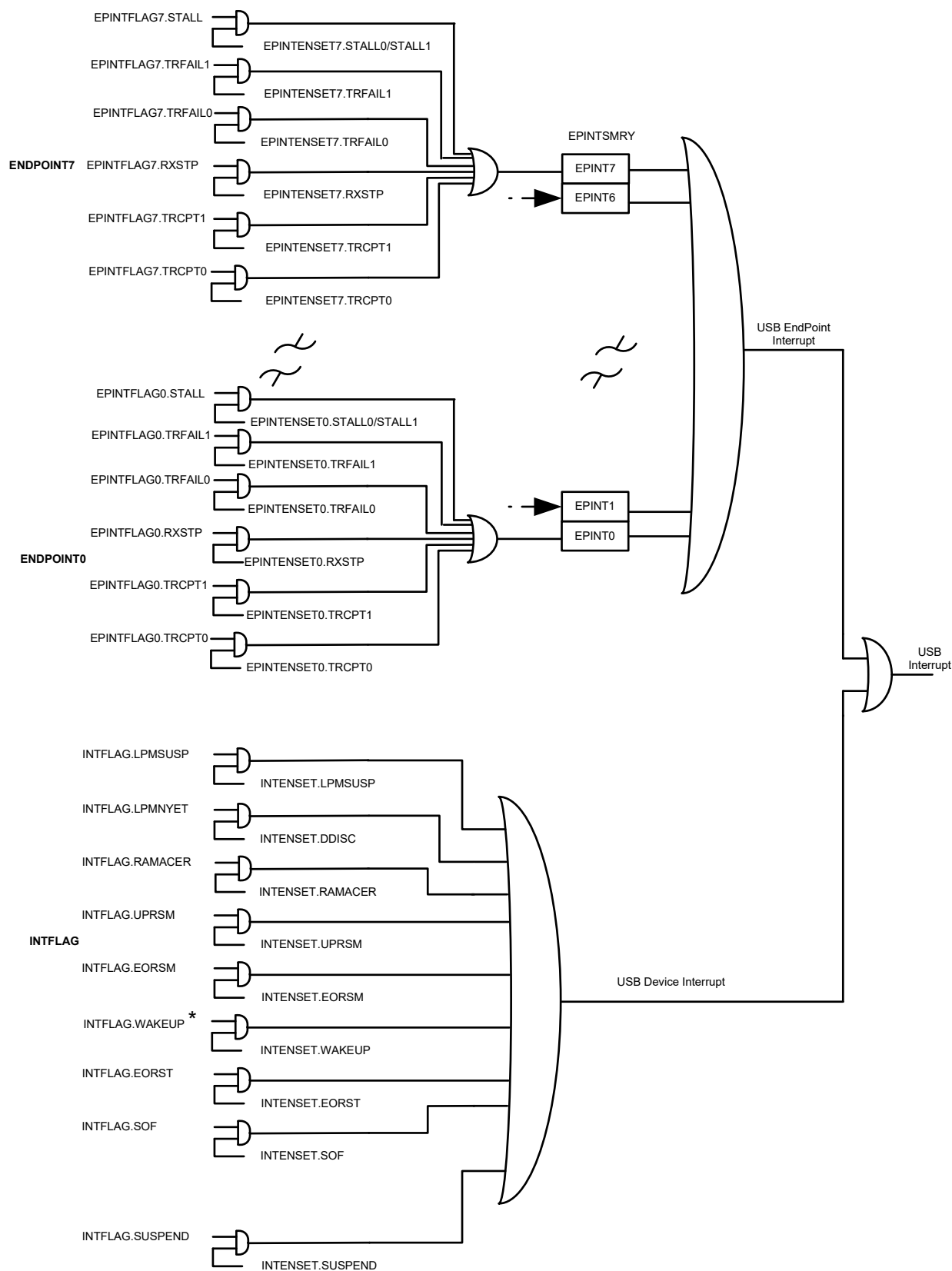
Figure 38-9. Device Interrupt
