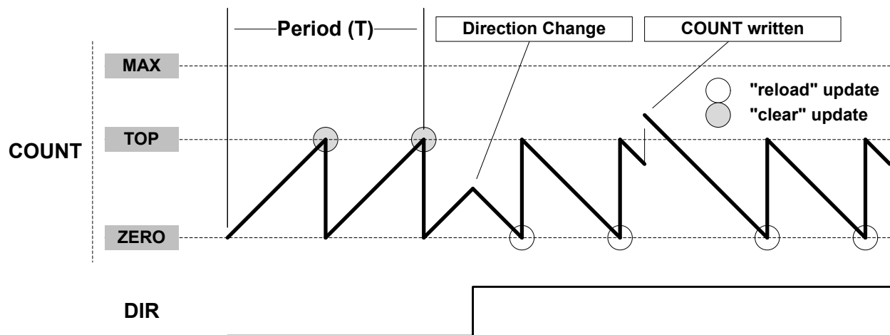
Figure 48-3. Counter Operation
