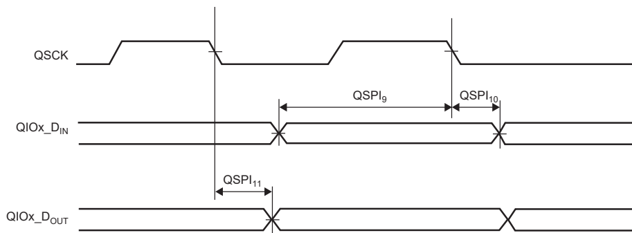
Figure 54-13. QSPI SDR Host Mode 3
