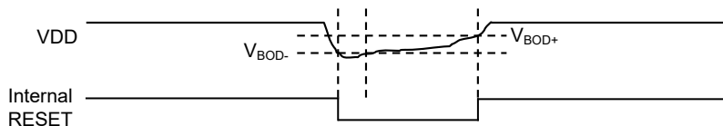
Figure 45-3. BODVDD Hysteresis ON
