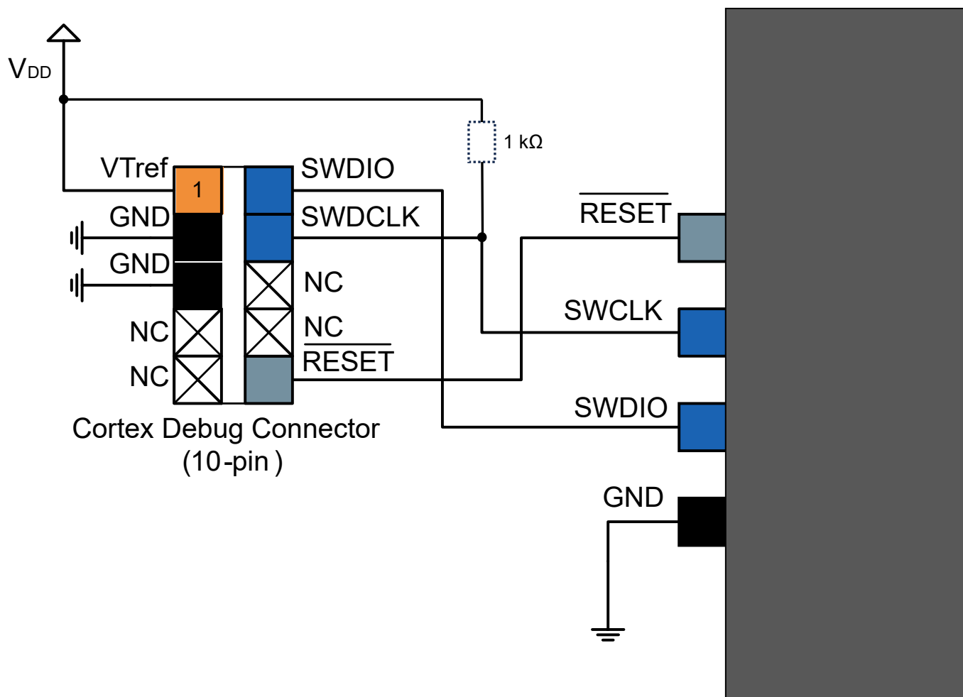
Figure 53-13. Cortex Debug Connector (10-pin)
