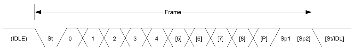
Figure 31-2. Frame Formats
