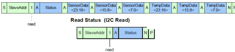
Figure 12. I2C Read Status
