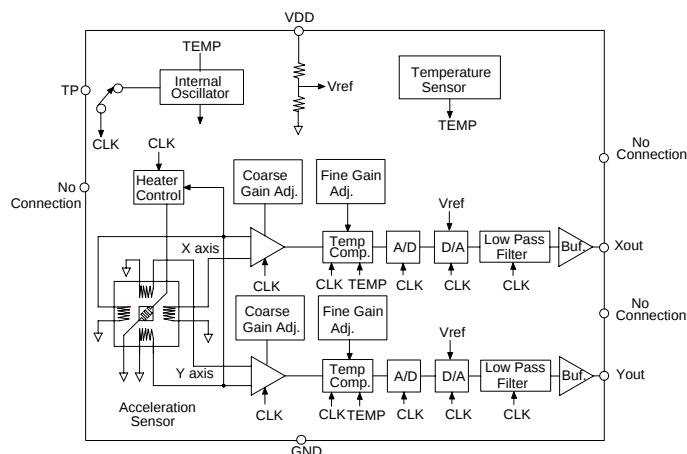
MXR7250VW FUNCTIONAL BLOCK DIAGRAM
