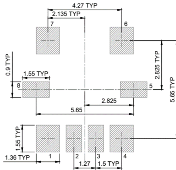
MXR7150VW Flat Mount
