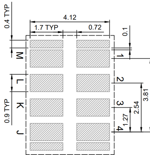
MXR7150VW Vertical Mount
