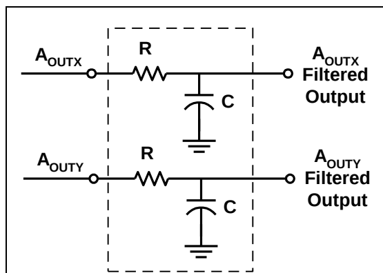
Figure 5: Low Pass Filter
