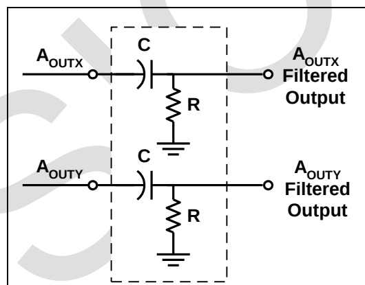
Figure 4: High Pass Filter
