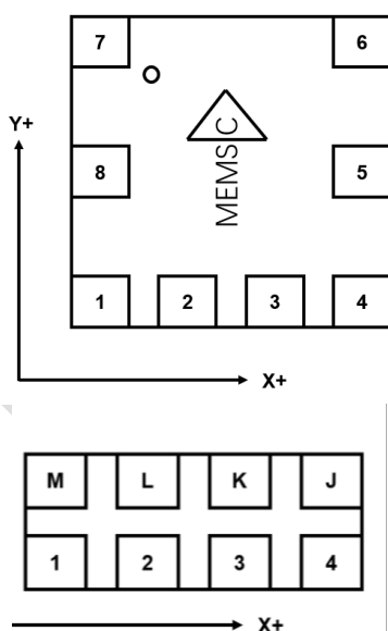
Figure 2: Sensing direction
