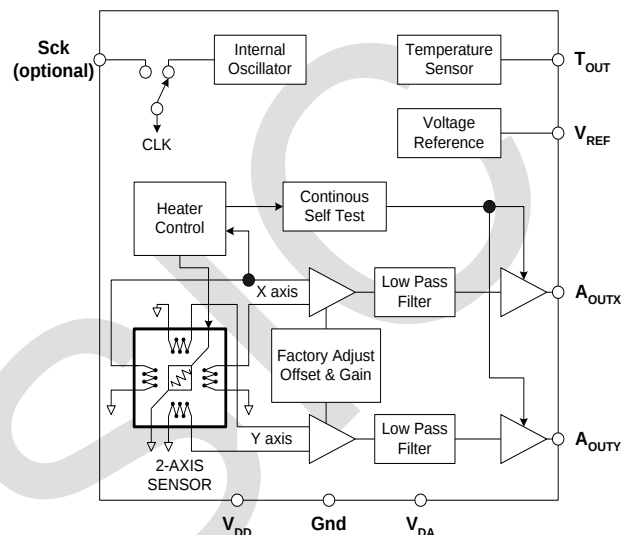
Figure 1: MXR2500MW functional block diagram
