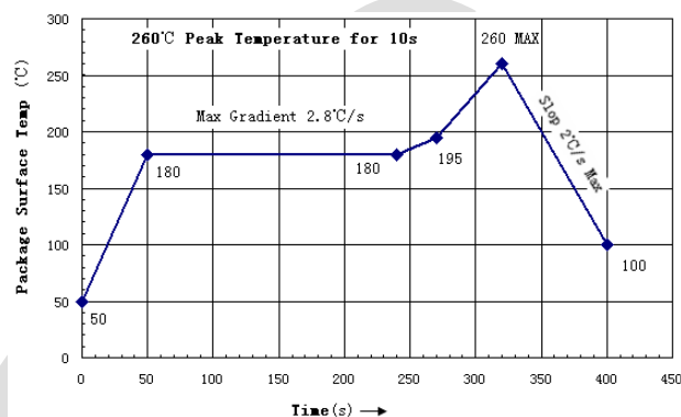
Figure 9: Recommended Reflow Solder Profile
