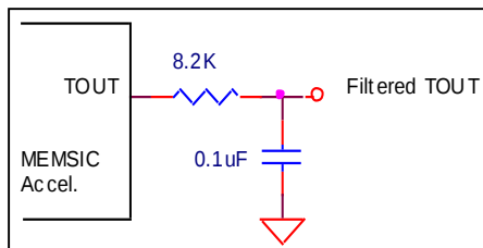
Figure 7: Temperature Output Noise Reduction
