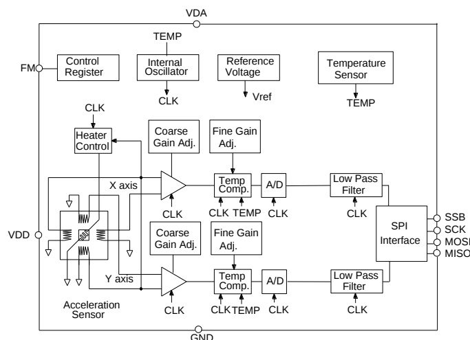
MXP7205VW FUNCTIONAL BLOCK DIAGRAM
