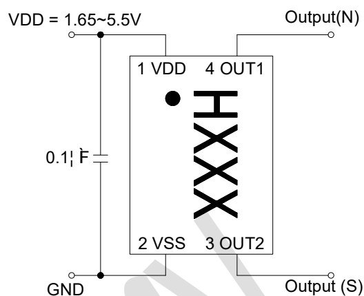
Figure 3: Connection diagram
