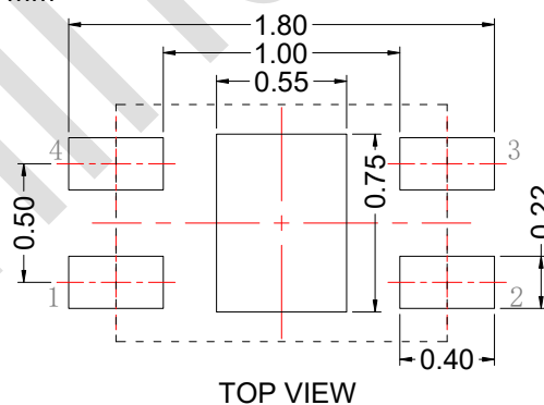
Figure 4: Recommended land pattern
