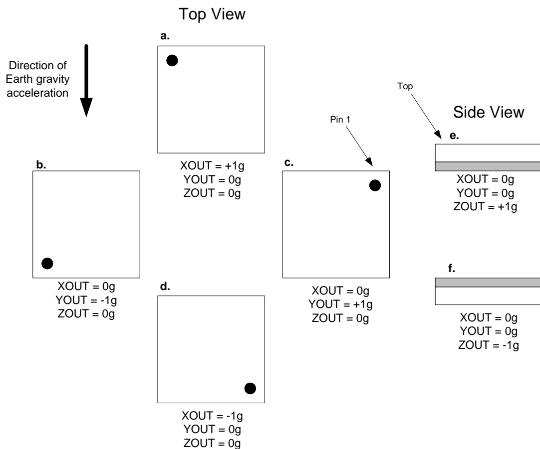
Figure 3. Package Orientation
