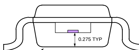
END VIEW
