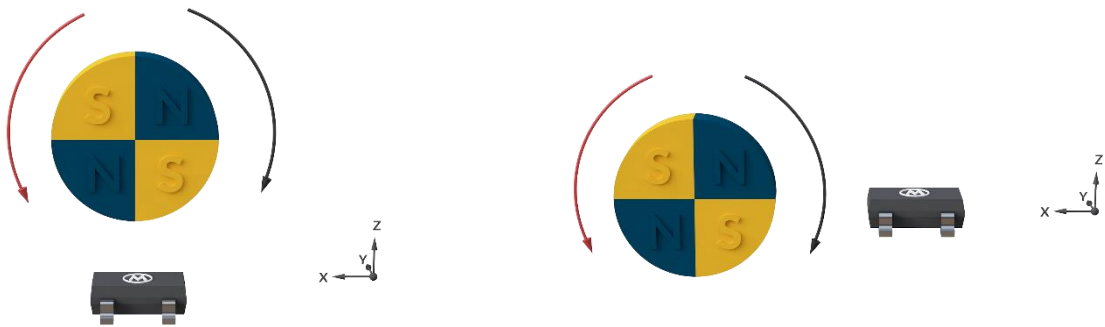
ZX configuration
