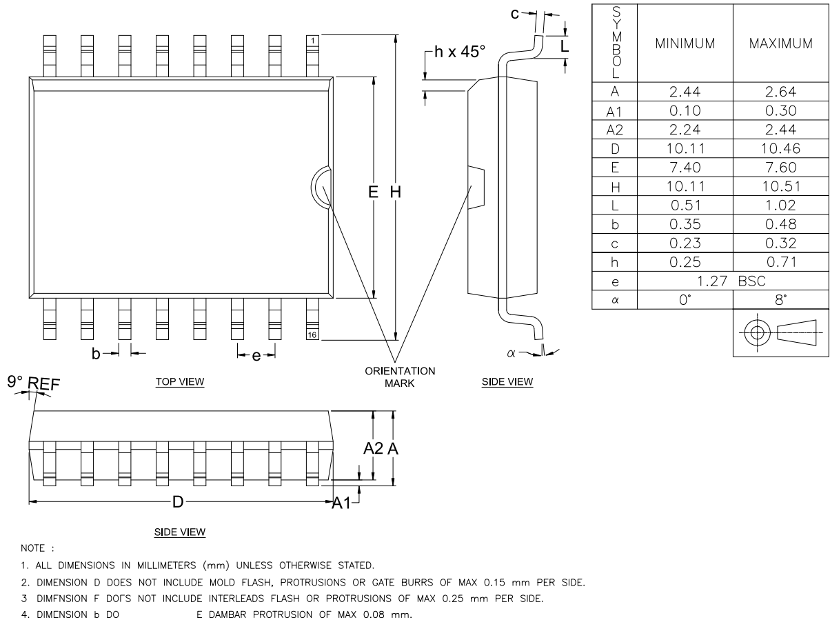
Figure 11: SOIC16 Package Dimensions
