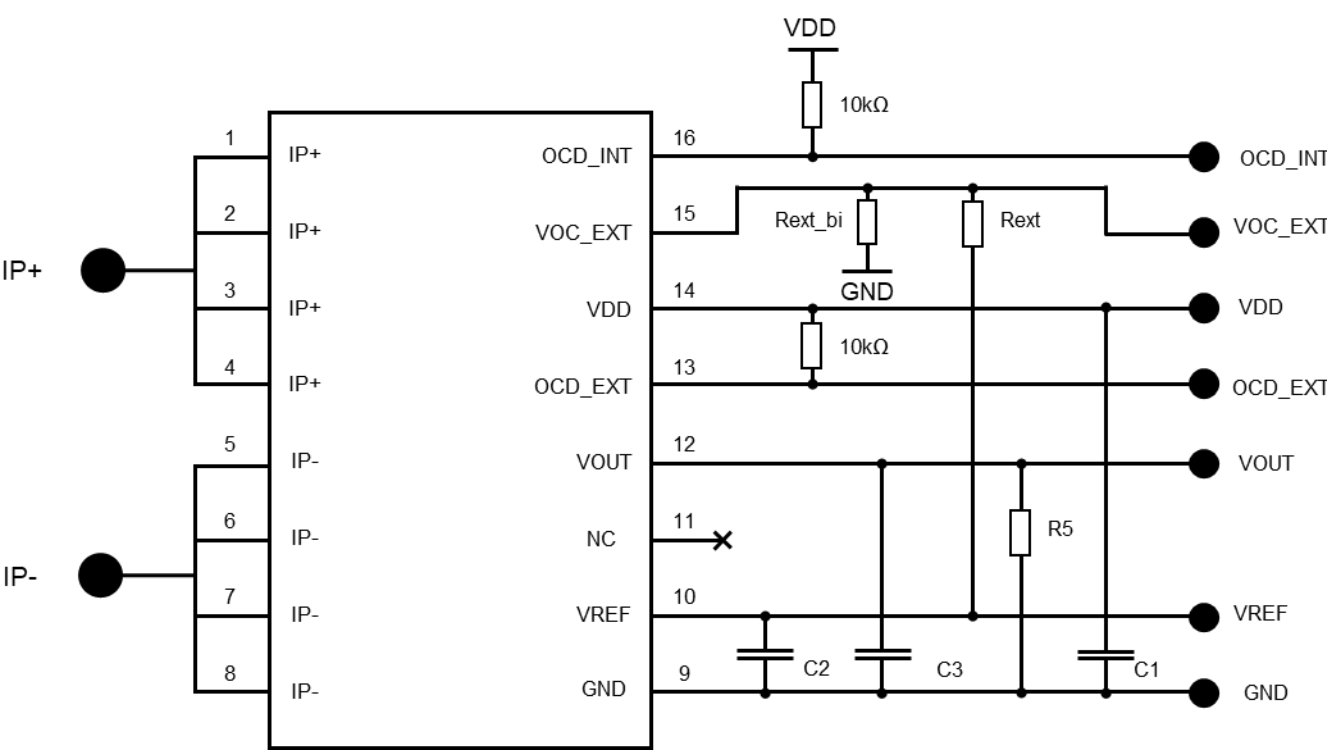
Figure 7: Recommended wiring for the MLX91220 with Bidirectional External OCD
