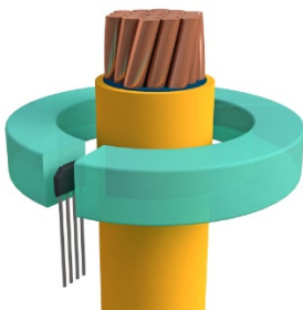
Figure 1. Typical Current Sensing Application
