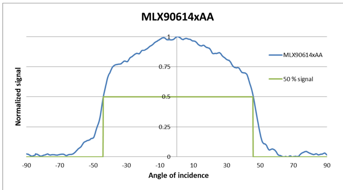
Figure 29: Typical FOV of MLX90614xAA
