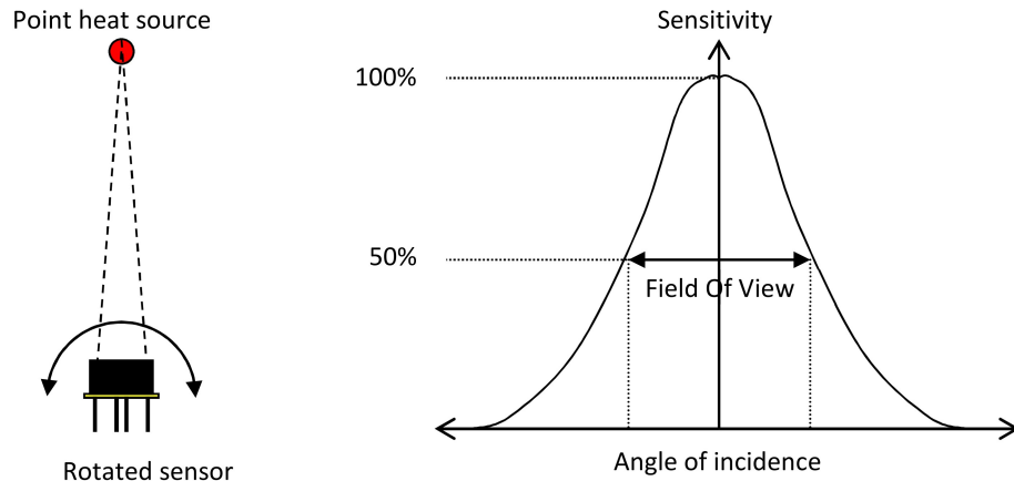
Figure 28: Field Of View measurement
