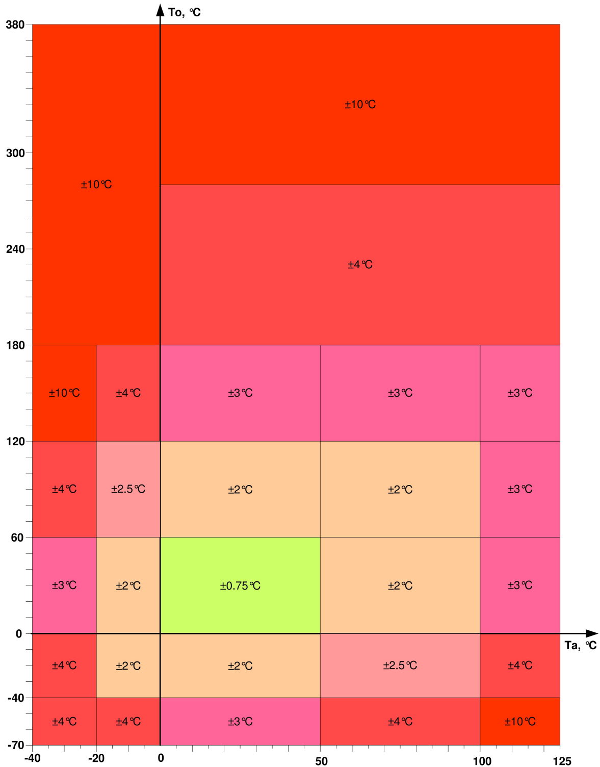
Figure 23 Accuracy of MLX90614xCK (Ta, To) only
