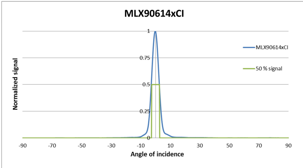
Figure 35: Typical FOV of MLX90614xCI
