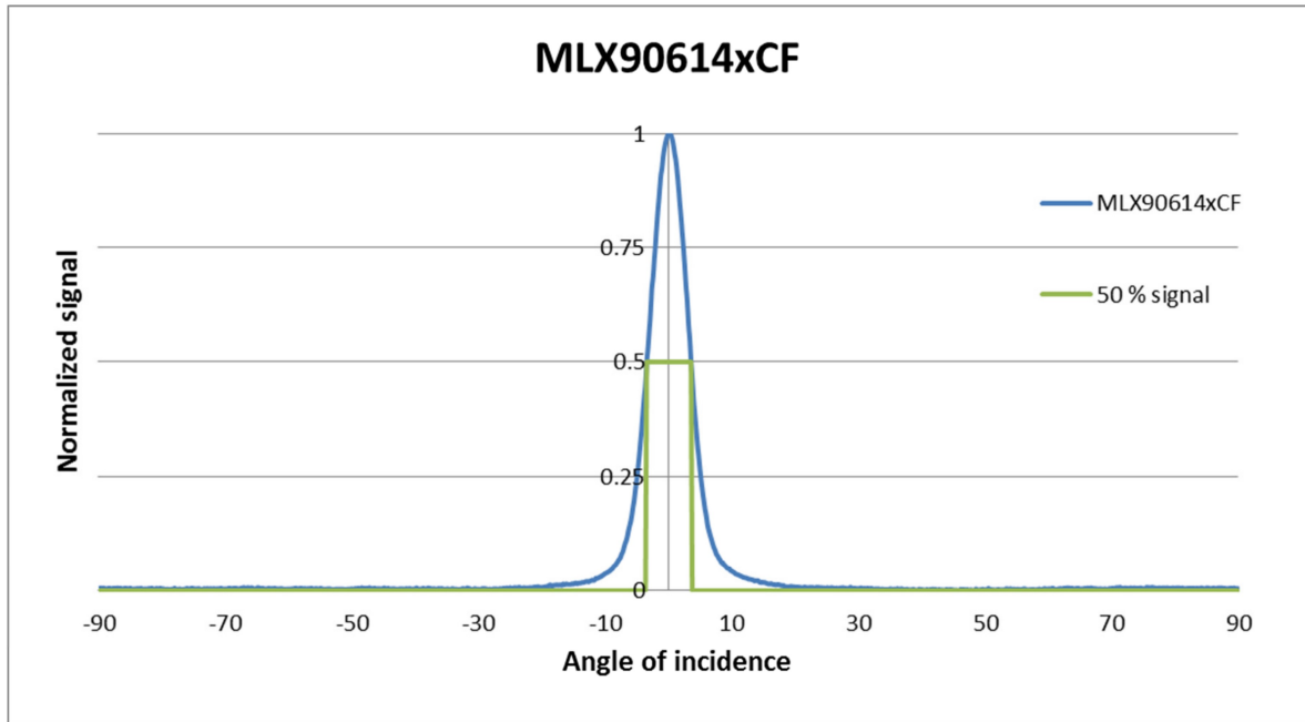
Figure 33: Typical FOV of MLX90614xCF
