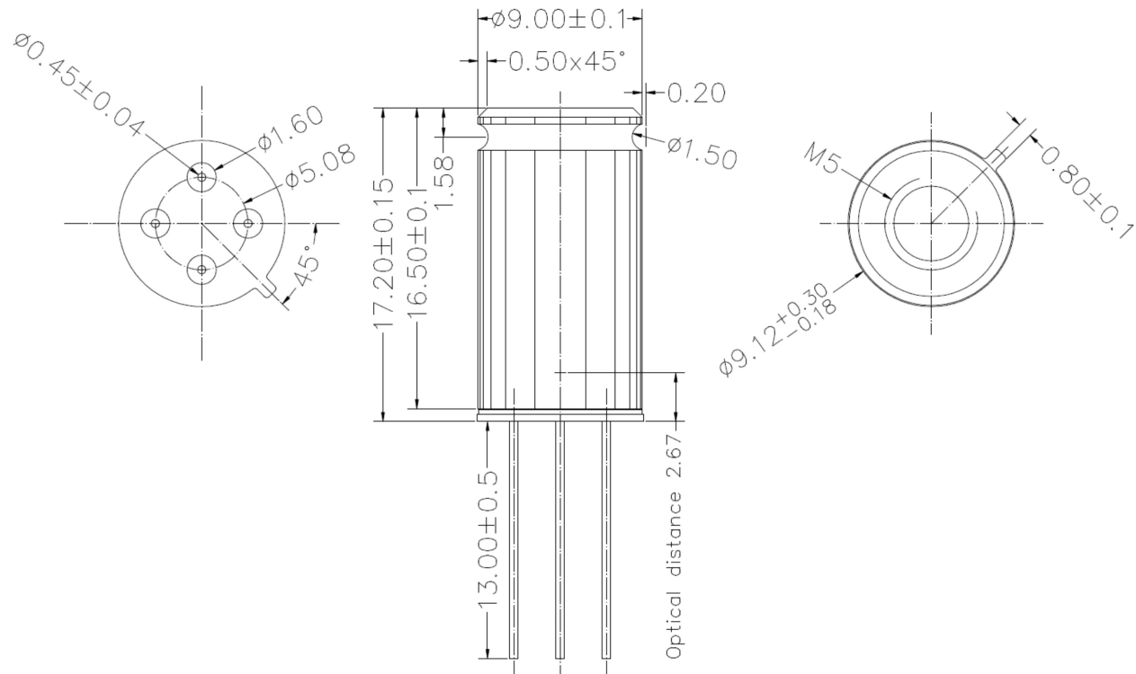
Figure 45: MLX90614xCF package
