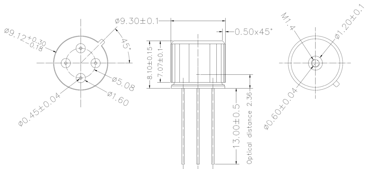
Figure 48 MLX90614xCK package
