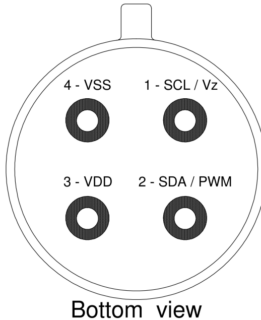
Figure 2: Pin description
