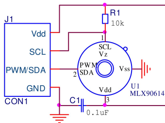
Figure 40: PWM output with SMBus available
