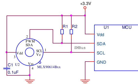
Figure 37: MLX90614 SMBus connection
