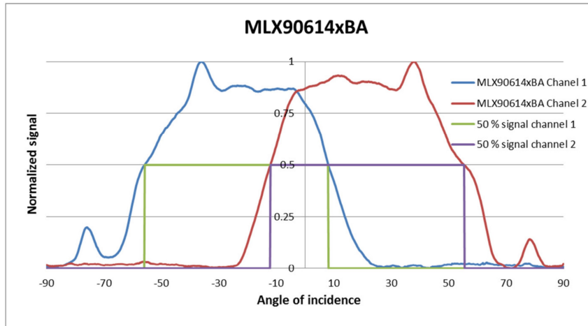
Figure 30: Typical FOV of MLX90614xBA
