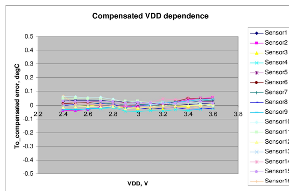
Figure 27: Typical To compensated dependence error
