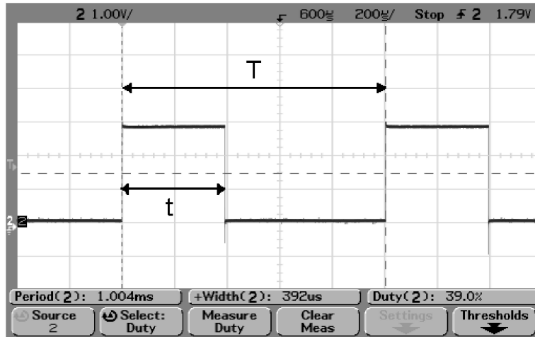
Figure 15: PWM example single mode
