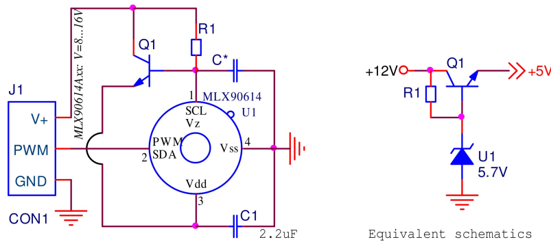
Figure 42: 12V regulator implementation
