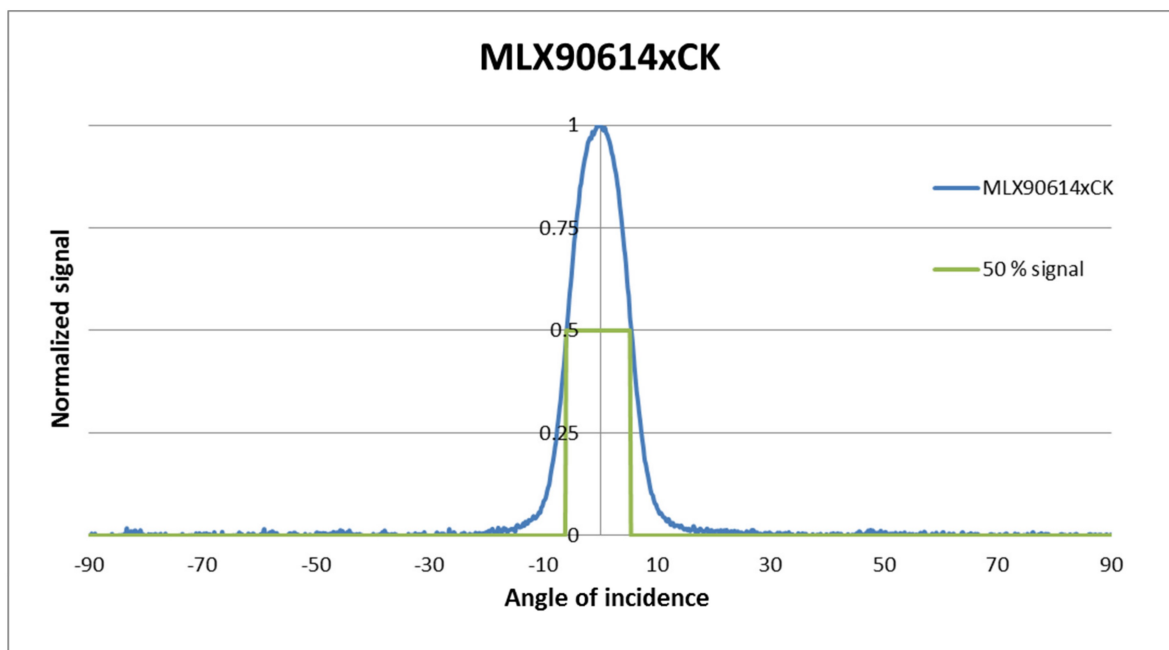
Figure 36 Typical FOV of MLX90614xCK type
