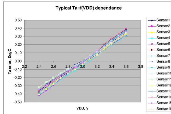
Figure 25: Typical Ta dependence from supply voltage
