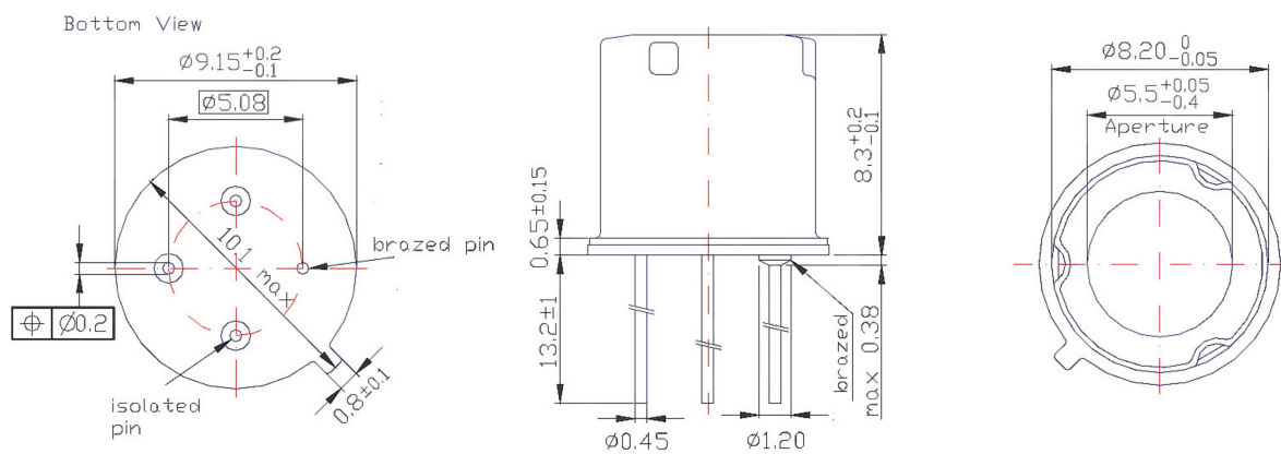
Figure 46: MLX90614xCH package
