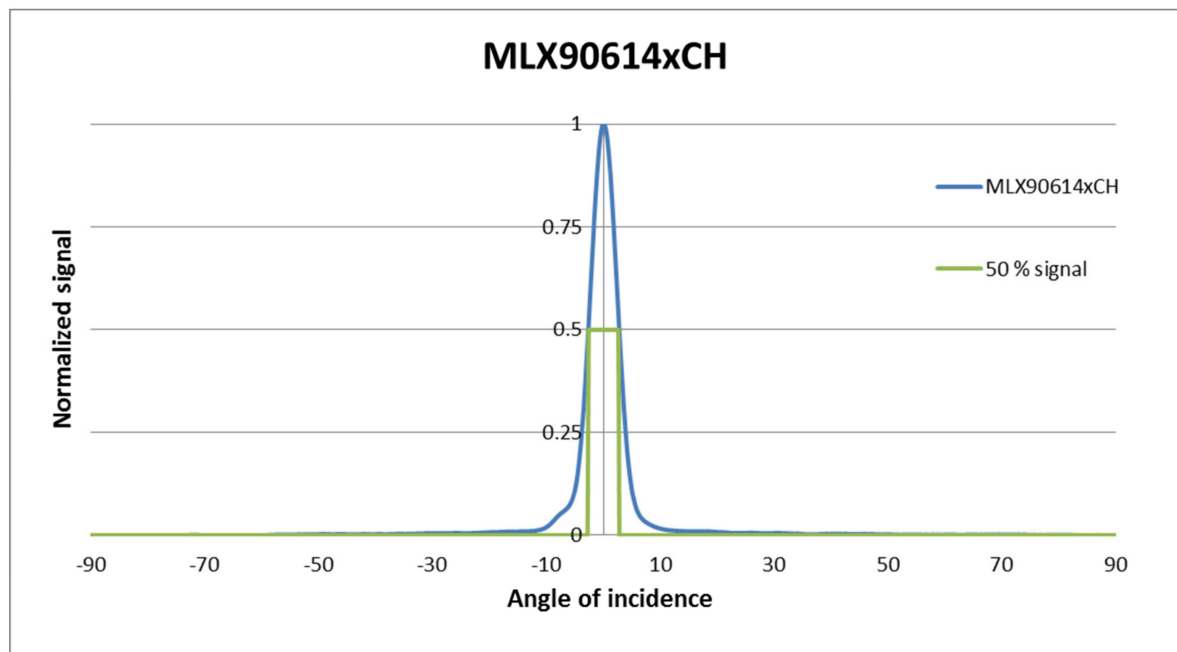
Figure 34: Typical FOV of MLX90614xCH
