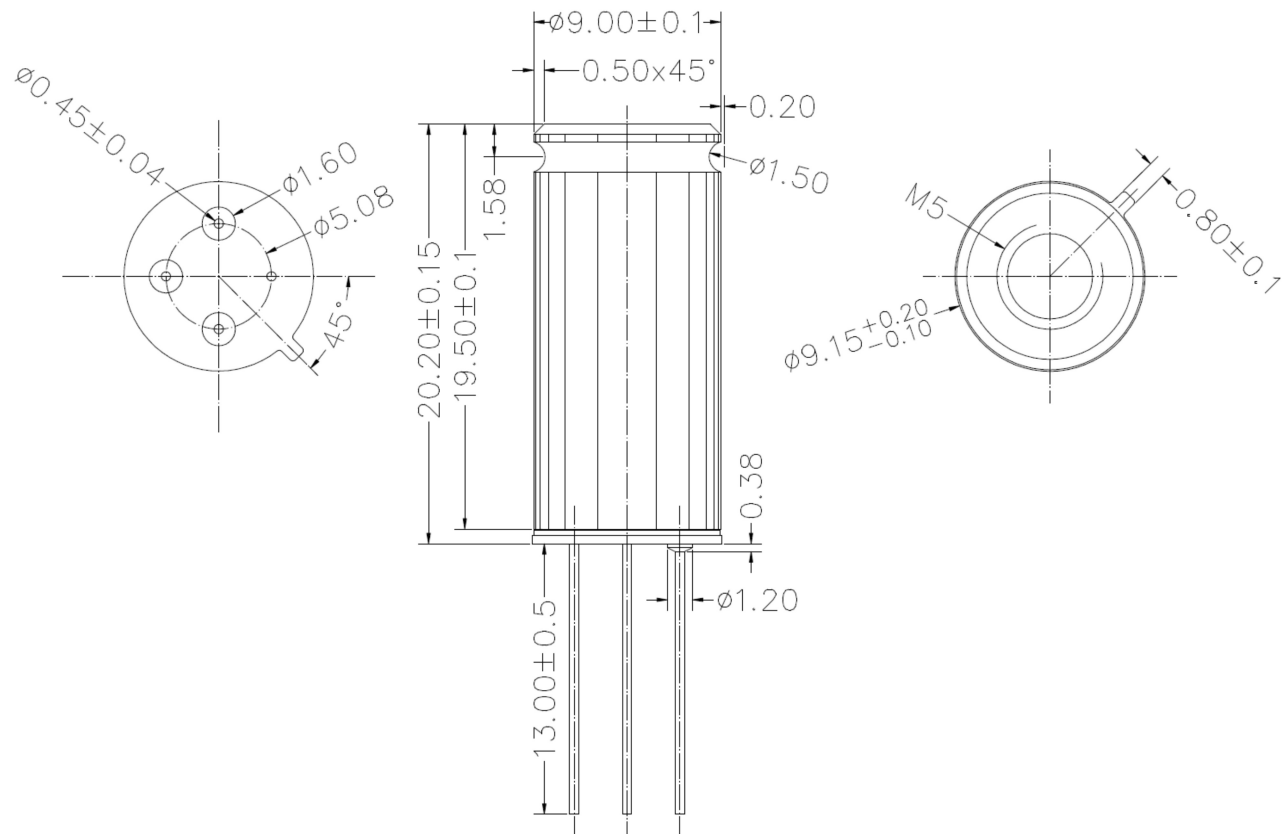
Figure 47: MLX90614xCI package
