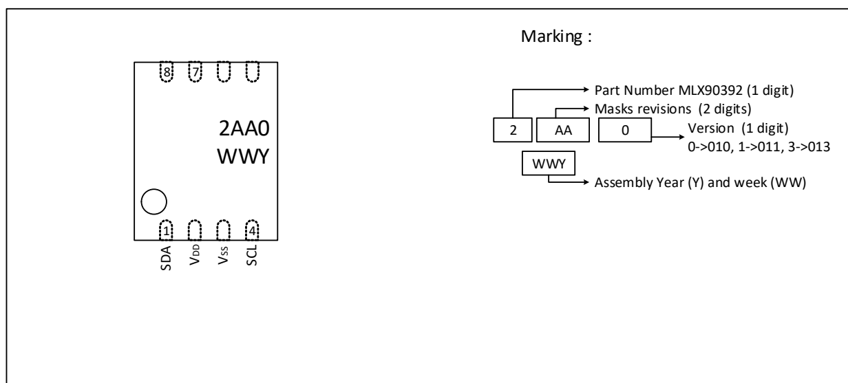
Figure 26: Marking
