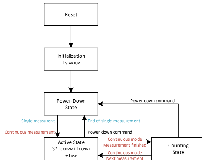
Figure 15: Sequence flowchart
