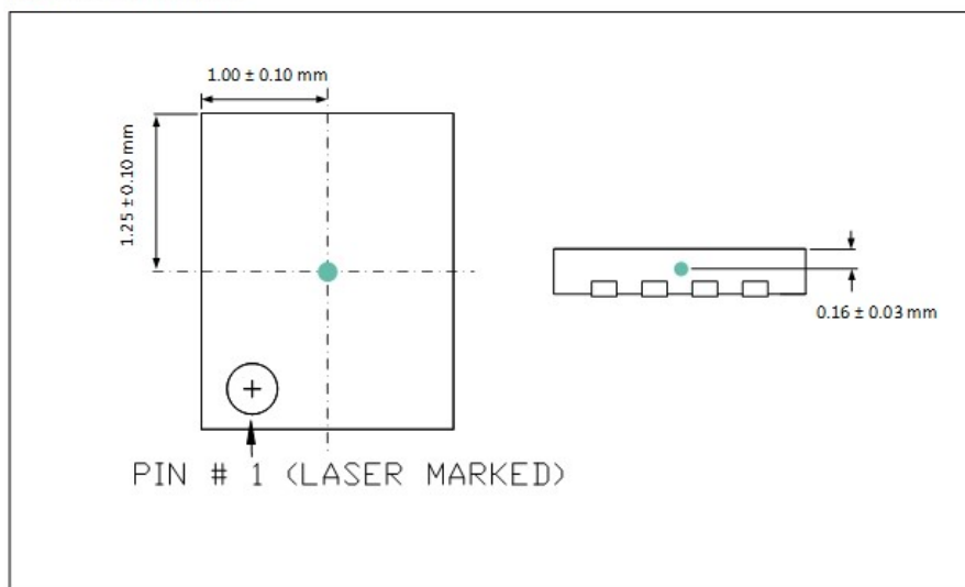
Figure 25: Field convention (Top view of the package with pin 1 at the bottom left)
