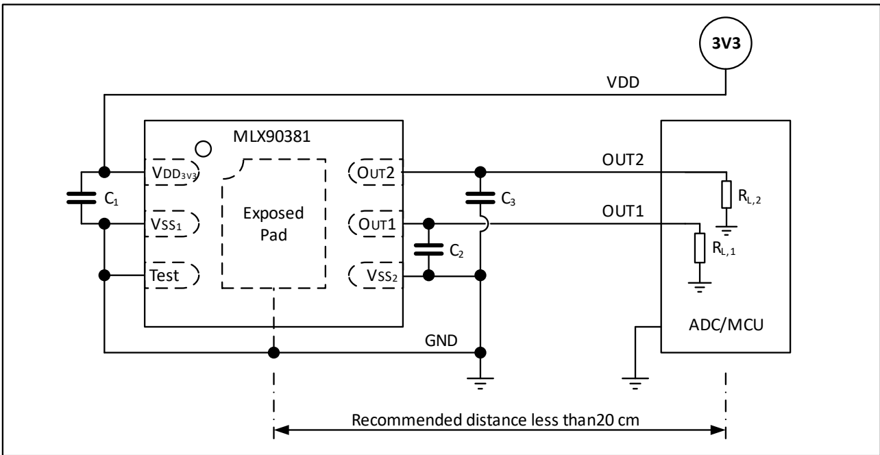
Figure 19 – Recommended application diagram
