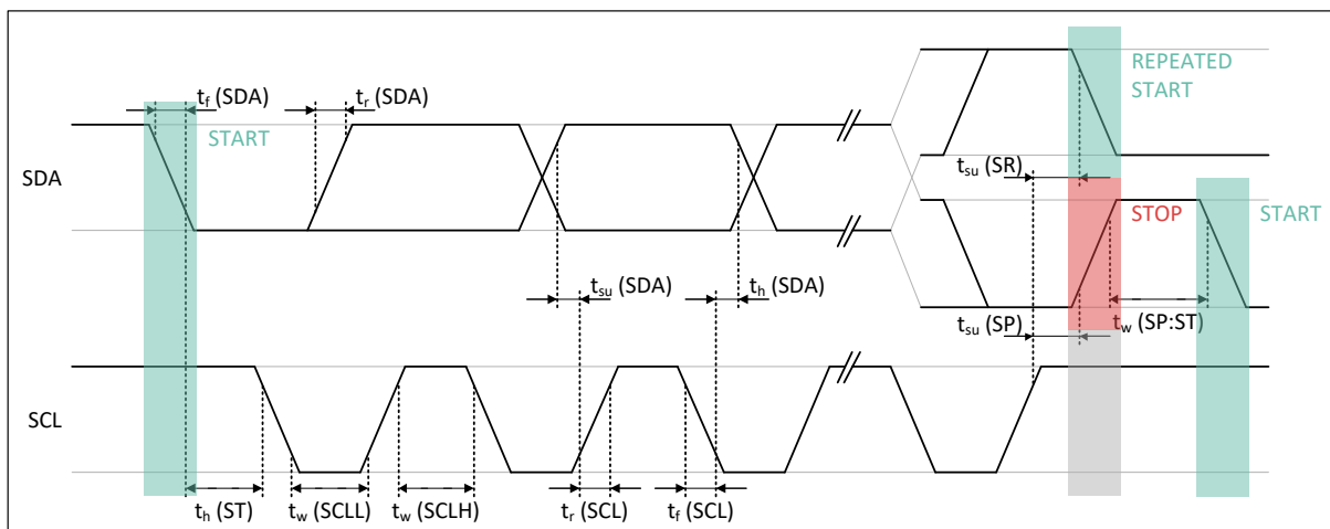
Figure 15 – I²C timing diagram
