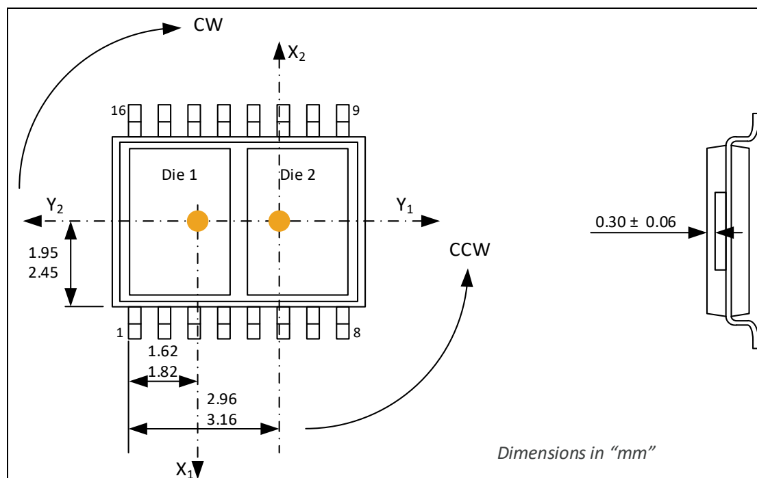
Figure 32 – TSSOP-16 Sensitive Spot Position
