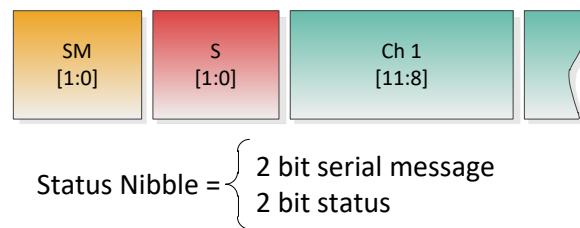
Figure 18 – SENT Status Nibble and Serial Message
