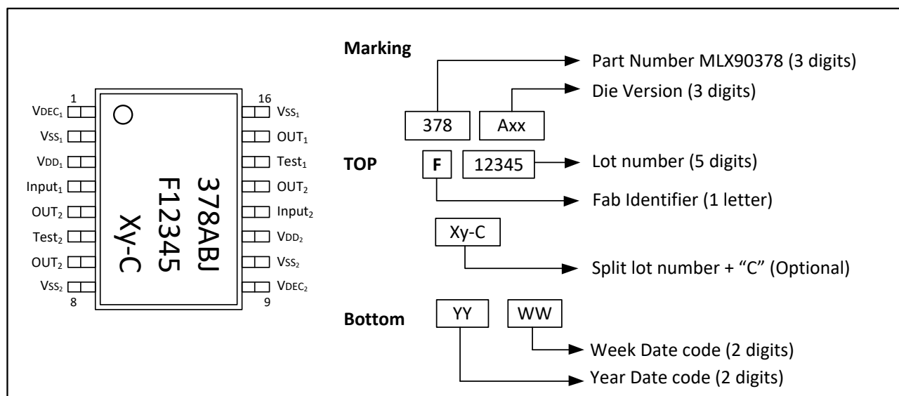
Figure 31 – TSSOP-16 Pinout and Marking
