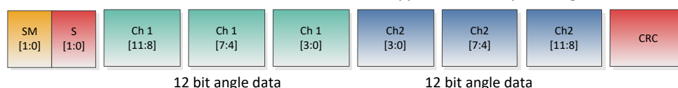
Figure 12 – A.7 Position Sensor Frame Format
