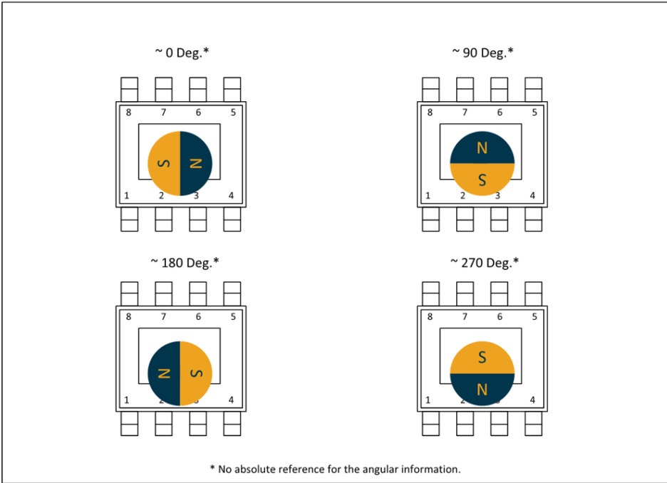
Figure 39 - SOIC-8 angle detection
