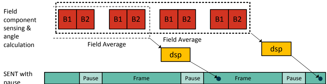
Figure 5 - Latency - Case FILTER = 2
