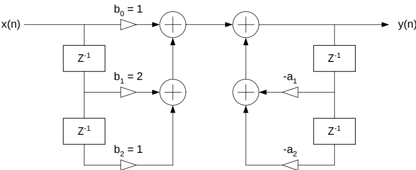
Figure 6 - IIR Diagram
