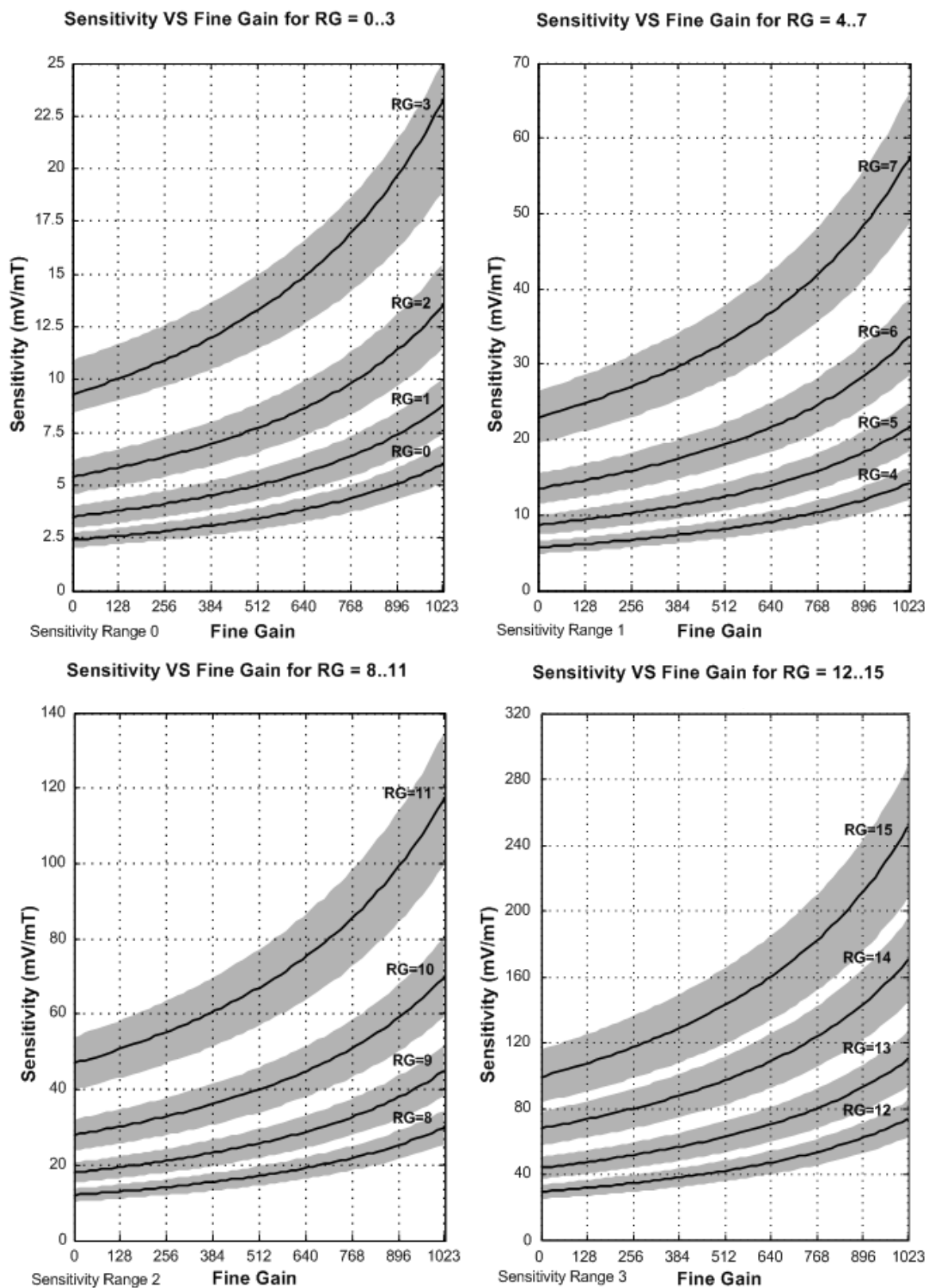
Figures 10.4-1...10.4-4 Sensitivity versus RG and FG. Important : You need option code 000 for Sensitivity Range 0 is option code 000, option code 1 for Sensitivity Range 1, option code 2 for Sensitivity Range 2 and option code 3 for Sensitivity Range 3.
