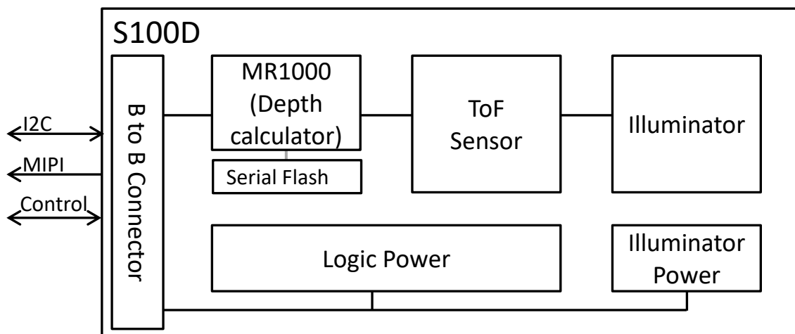
Fig 8. S100D system block diagram
