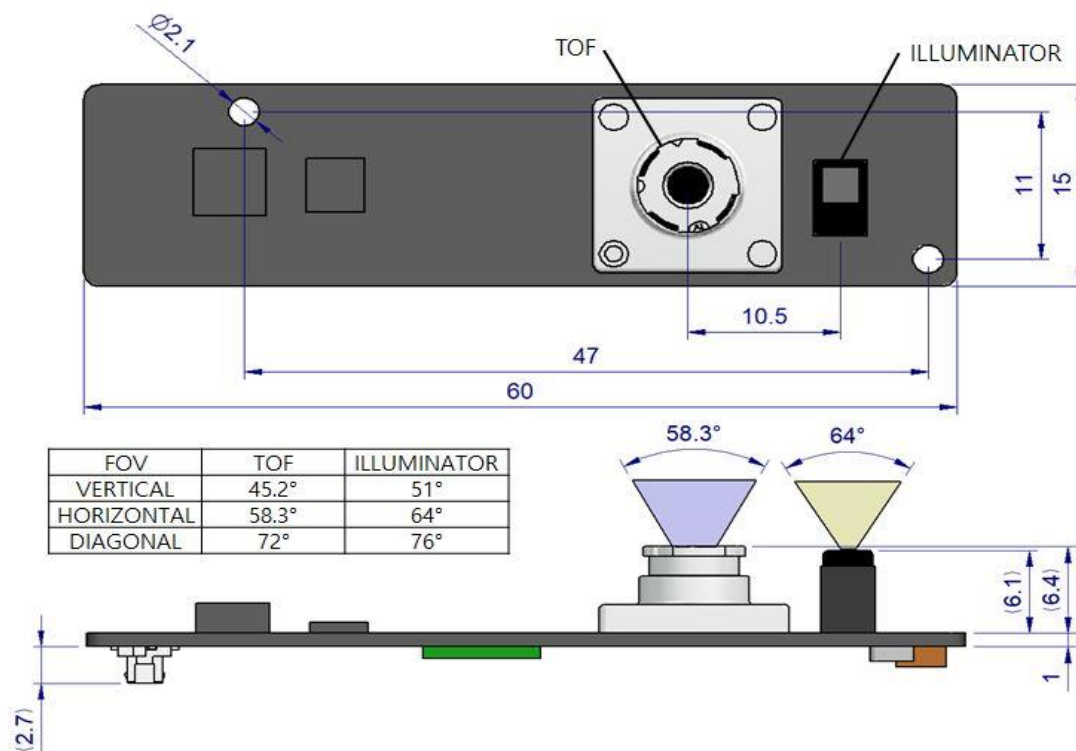
Fig 12. S100D dimension and schematic
