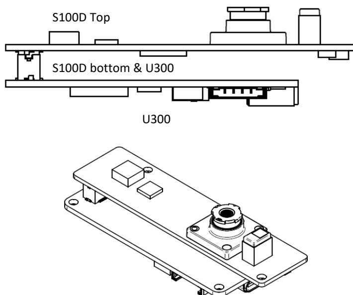
Fig 19. Combined S100D and U300
