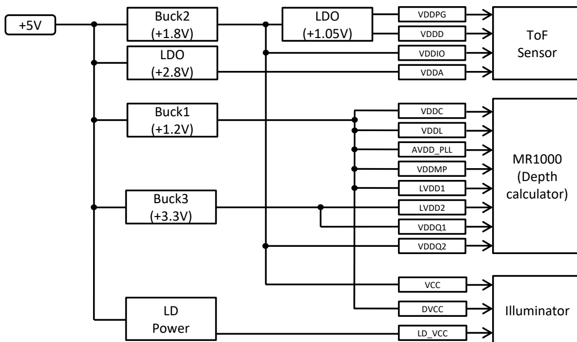
Fig 9. S100D system power
