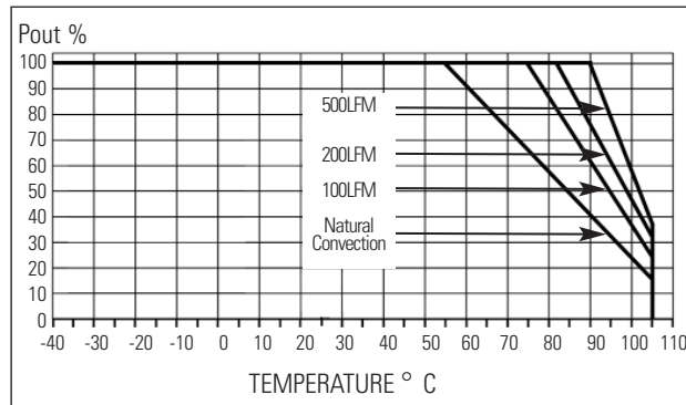
MODEL 2703SXX (With heatsink)
