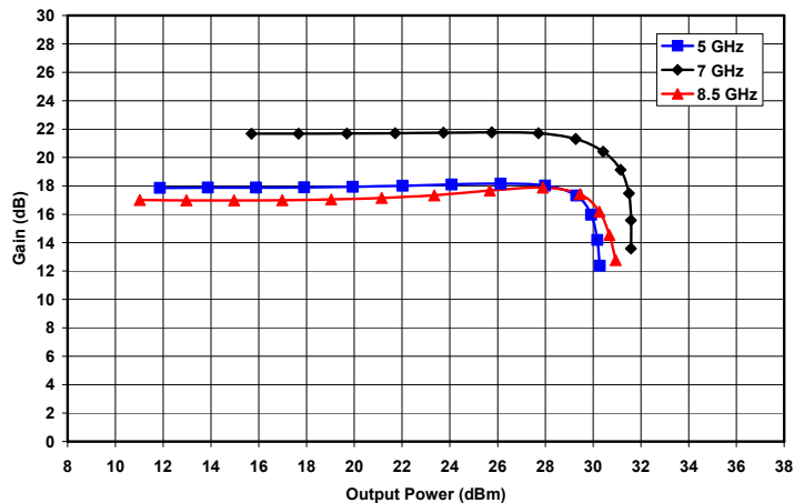
Figure 8. Gain vs. Output Power and Frequency at VD = 6V and IDQ = 600mA
