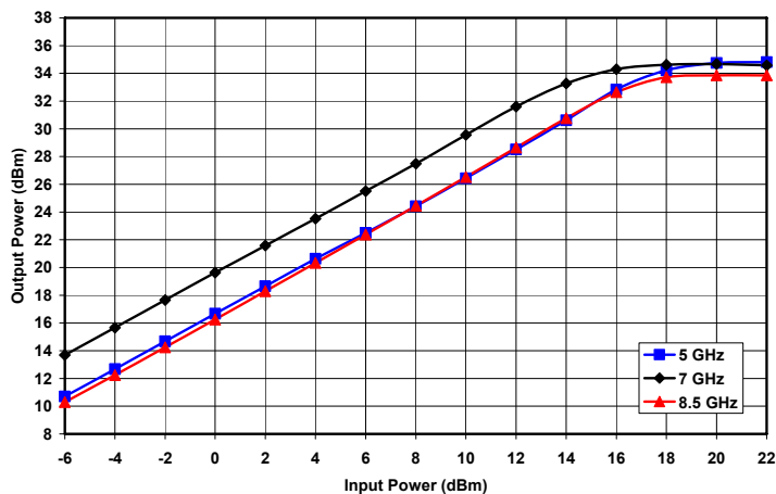
Figure 11. Output Power vs. Input Power and Frequency at VD = 10V and IDQ = 600mA
