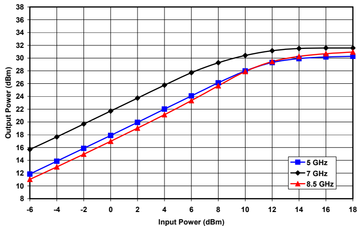
Figure 7. Output Power vs. Input Power and Frequency at VD = 6V and IDQ = 600mA
