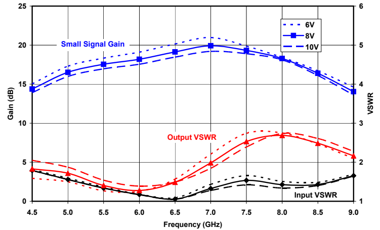
Figure 2. Small Signal Gain and Input & Output VSWR vs. Frequency and Drain Voltage at IDQ = 600mA
