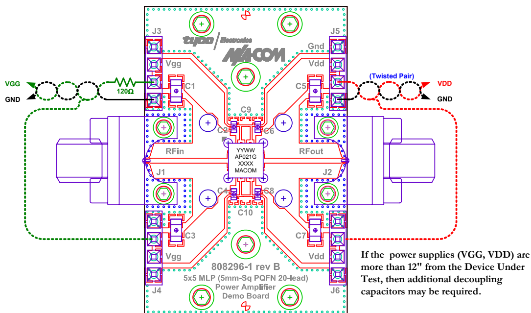
Figure 29. Demonstration Board PN MAAP-000021-SMB003 (available upon request).
