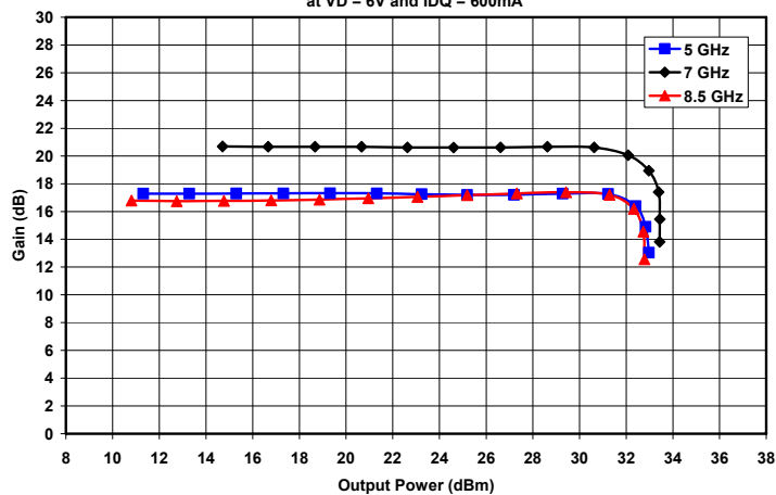
Figure 10. Gain vs. Output Power and Frequency at VD = 8V and IDQ = 600mA
