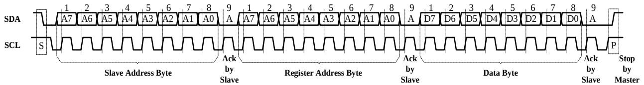
Figure 5-3 Writing to IS32SE5117A
