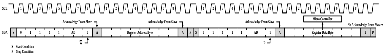
Figure 5-4 Reading from IS32SE5117A
