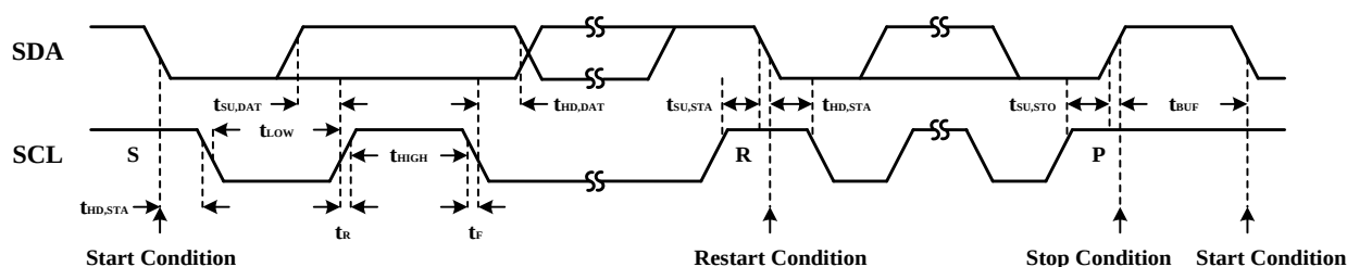
Figure 5-1 Interface Timing
