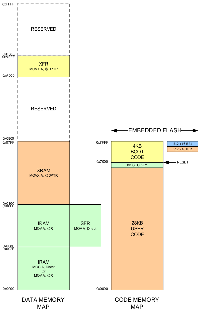
Figure 2-1 Memory Map
