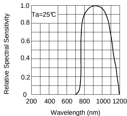
FIG.1 SPECTRAL SENSITIVITY
