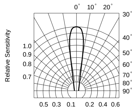
FIG.6 SENSITIVITY DIAGRAM
