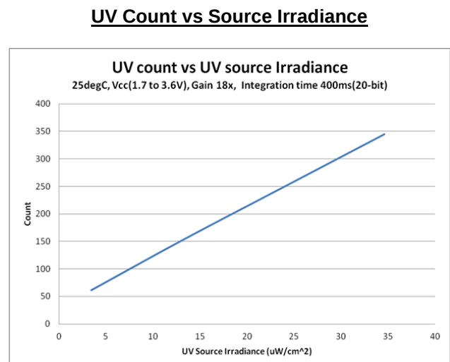
Figure 4.4 UV Count vs Source Irradiance
