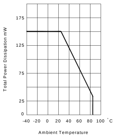
Fig.8 TOTAL POWER DISSIPATION VS AMBIENT TEMPERATURE
