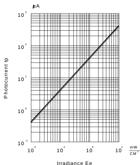
Fig.6 PHOTOCURRENT I_p VS IRRADIANCE E_e \lambda = 940 nm
