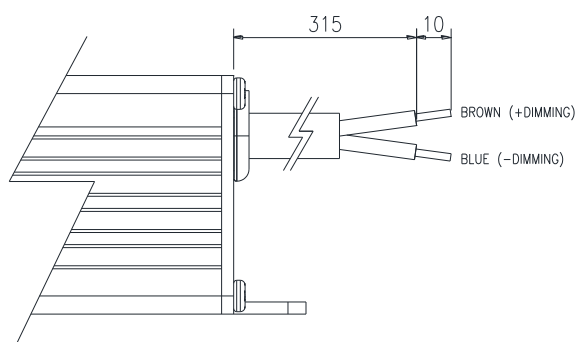
Detail "A"
