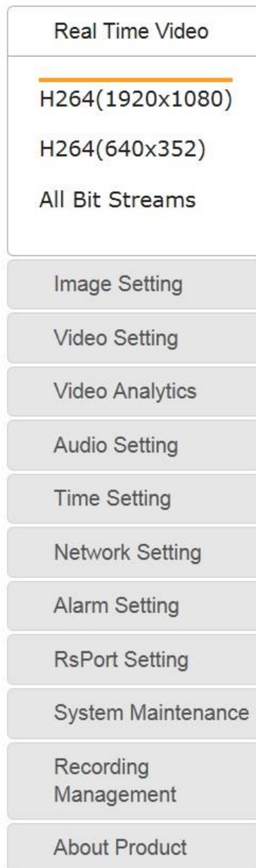
Figure 5: Navigation Interface
