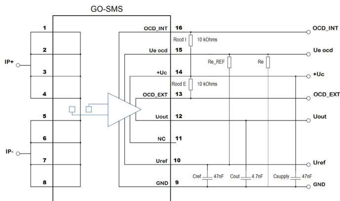
Figure 2: Application circuit
