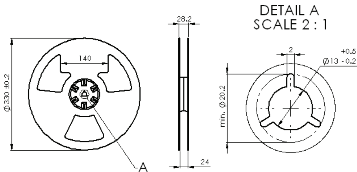
Figure 20: Plastic reel
