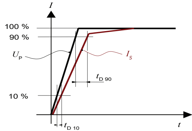
Figure 19: Delay time t_{D90} @ 90 and delay time t_{D10} @ 10
