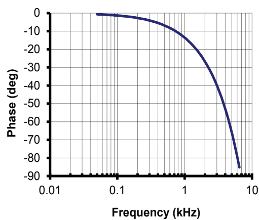
Figures 11 and 12: Typical frequency and phase response (detail)
