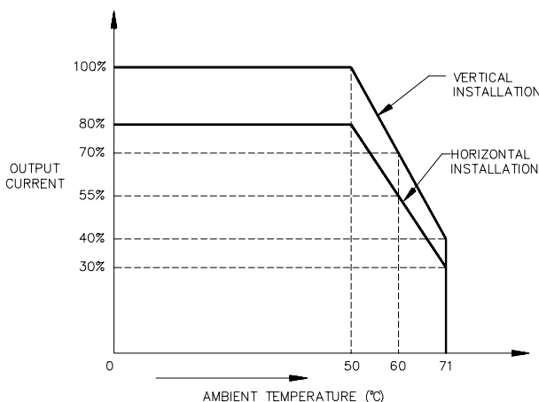
FIGURE 1. TEMPERATURE DERATING
