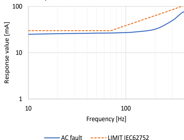
Frequency Characteristics of Response Value ( FG-R02-4BA )
