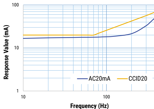
Frequency Characteristics of Response Value ( FG-R02-4A )
