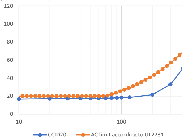
Frequency Characteristics of Response Value ( FG-R02-4GA )
