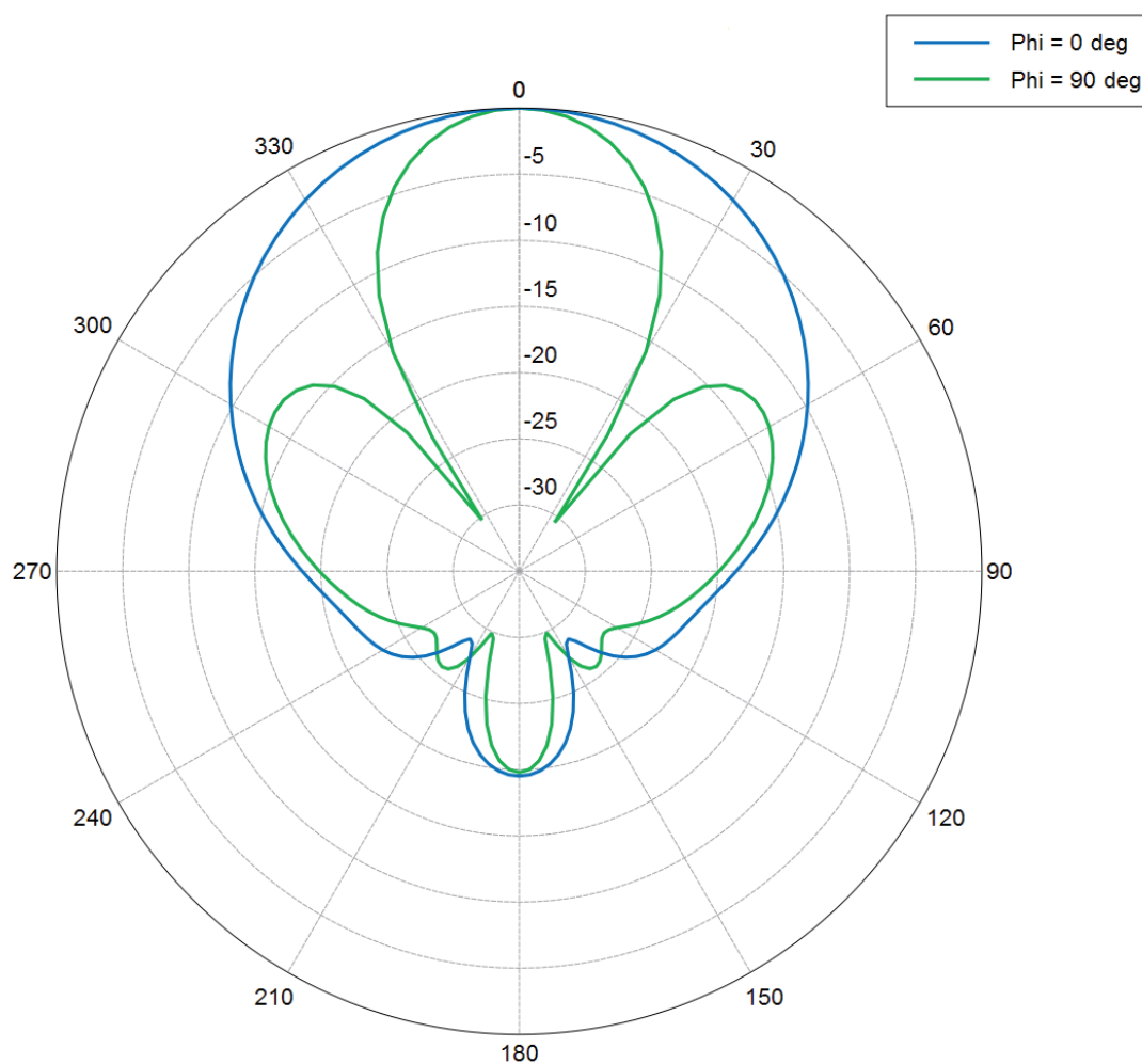
Figure 21: Antenna diagram WIRA-30-circular
