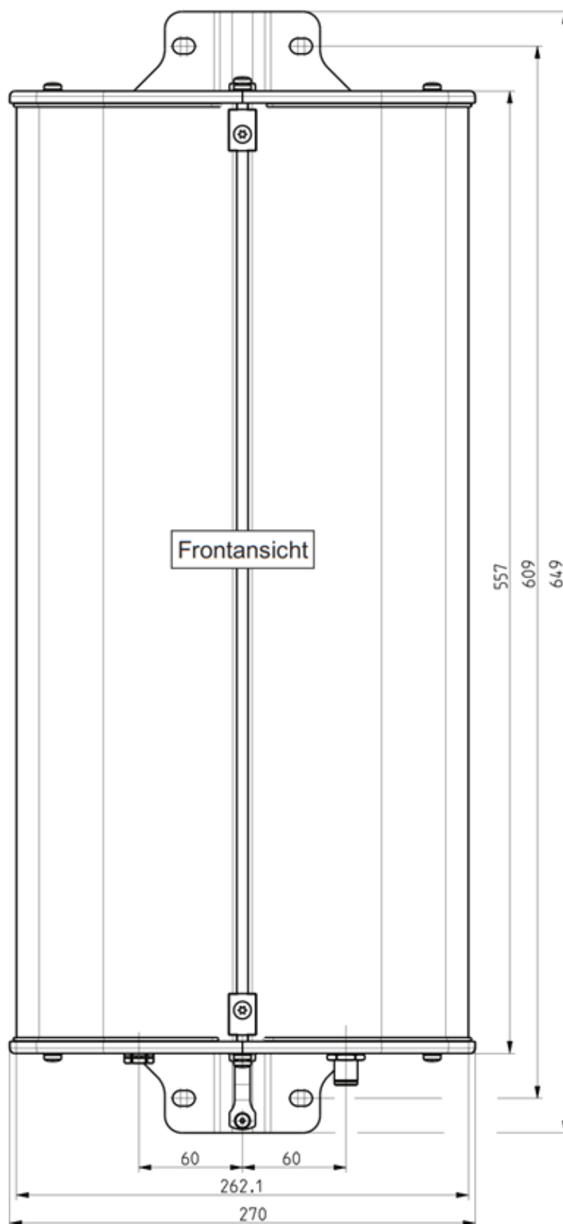
Figure 34: Dimensions for WIRA 30° antenna (52010086, -87)
