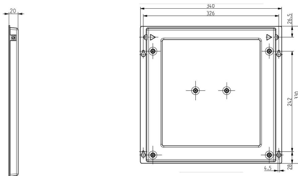
Figure 37: Dimensions for SSMH antenna/-modul (52010219, -258, -259, -260)
