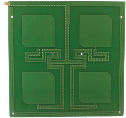
Figure 6: SMSH without protective cover
