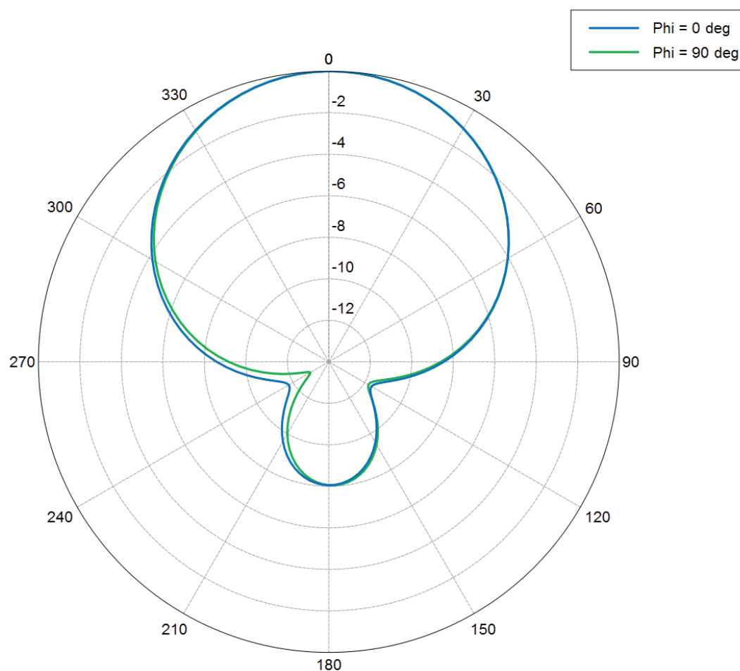
Figure 15: Antenna diagram MIRA-100-circular
