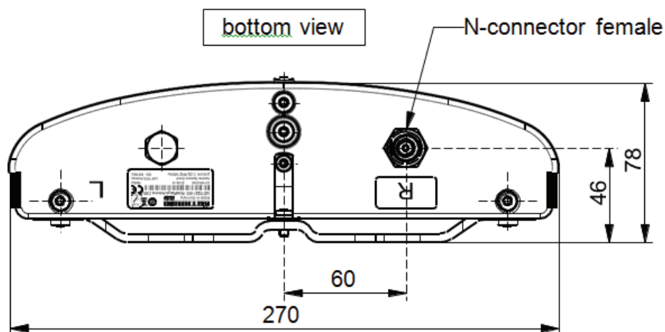
Figure 35: Note left / right installation WIRA-30-CSB-KRAI antenna (52010227, -228)
