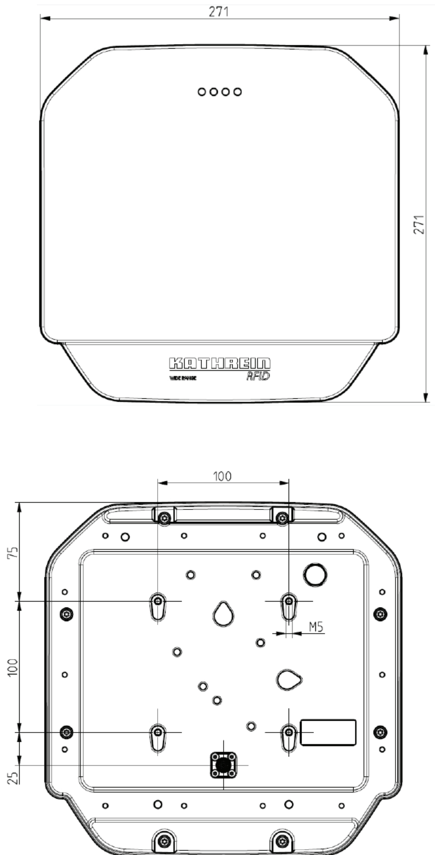
Figure 32: Dimensions for WIRA 70° antenna (52010078, -79)
