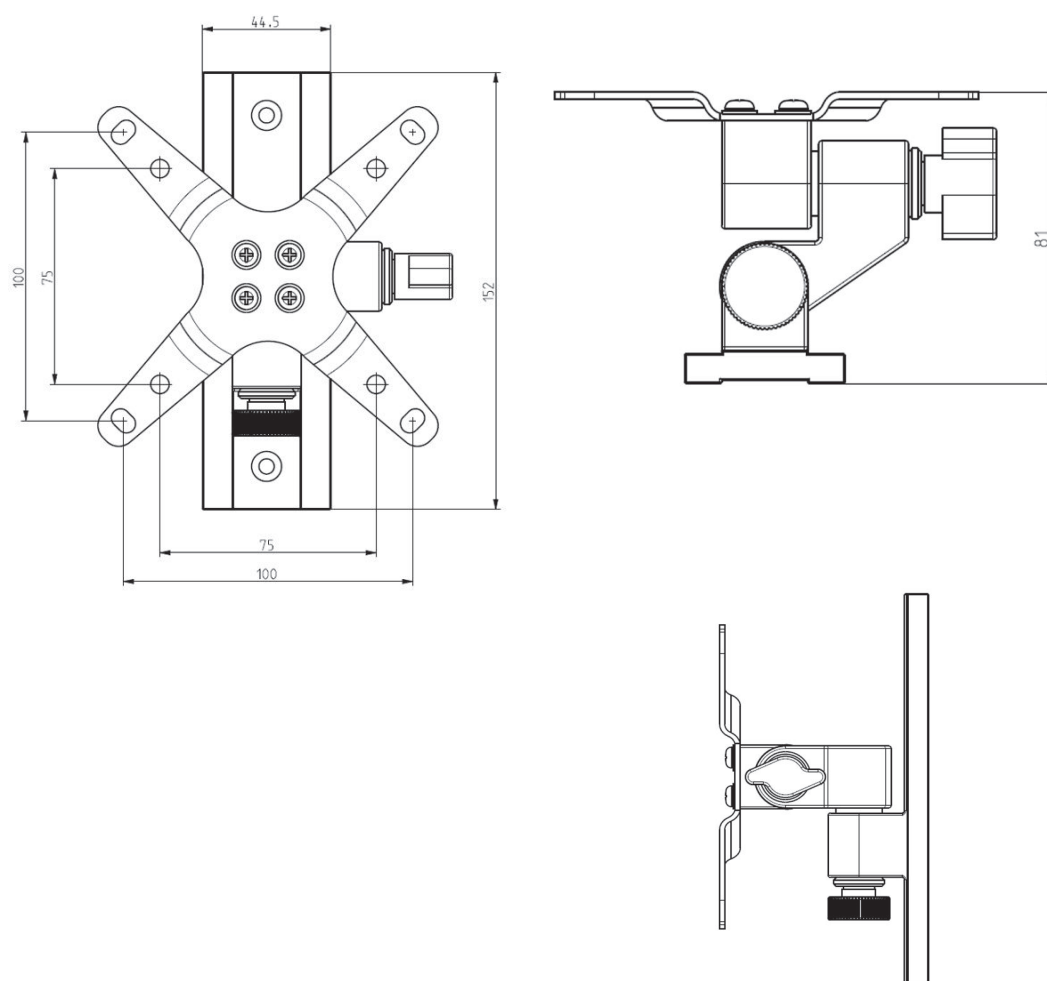
Figures 29: Wall mounting set 52010261
