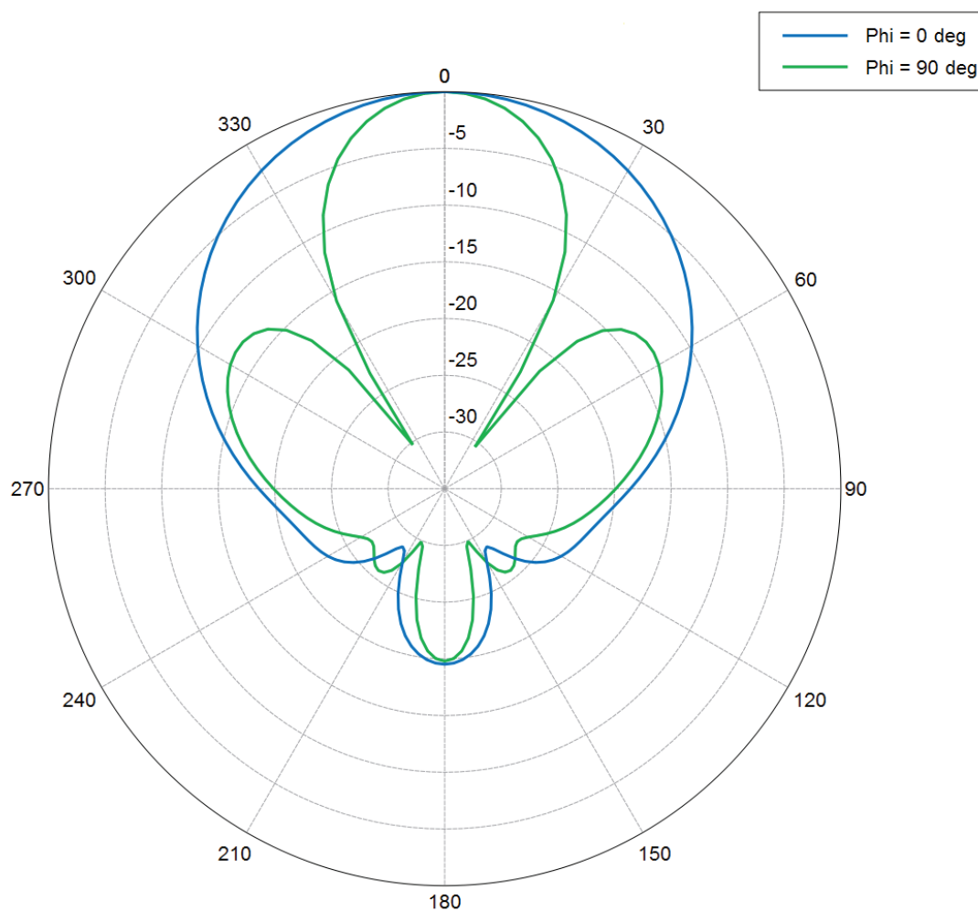
Figure 20: antenna diagram WIRA-30-linear
