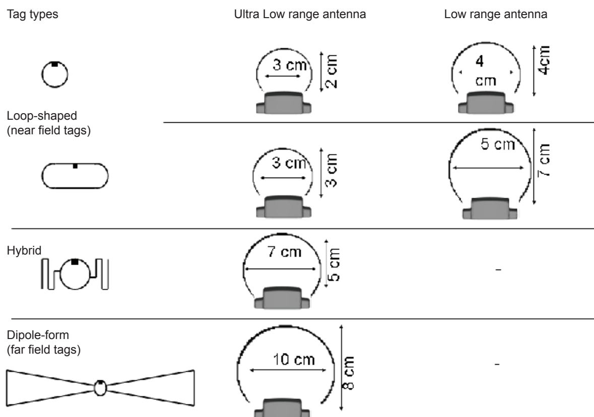
Figure 13: Read ranges of LORA and U-LORA by tag antenna
