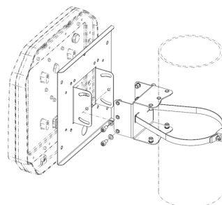
Figures 27: Wall/Pole mounting set 52010128
