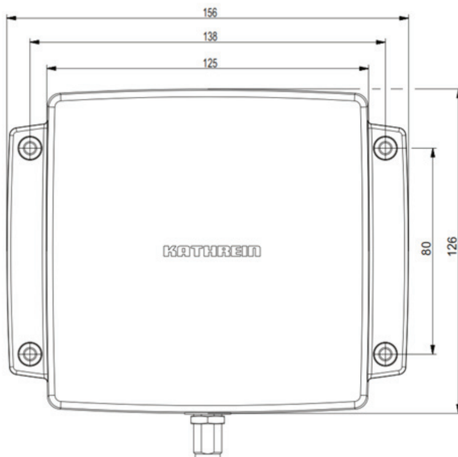
Figure 31: Dimensios for MIRA/S-MIRA antenna (52010172, -82, -83)
