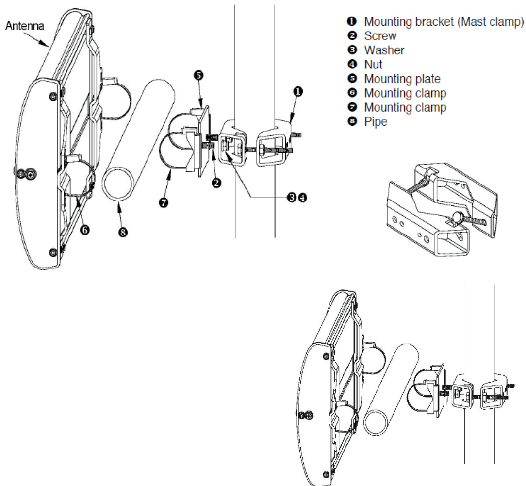
Figures 28: Pole mounting set 52010005
