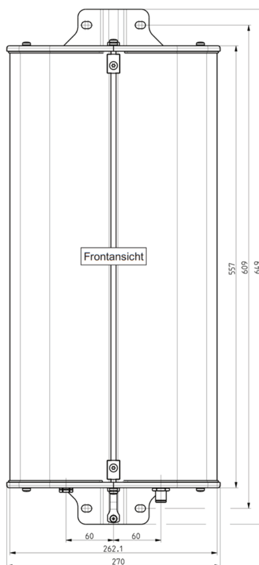
Figure 36: Dimensions for WIRA-30-CSB-KRAI antenna (52010227, -228)
