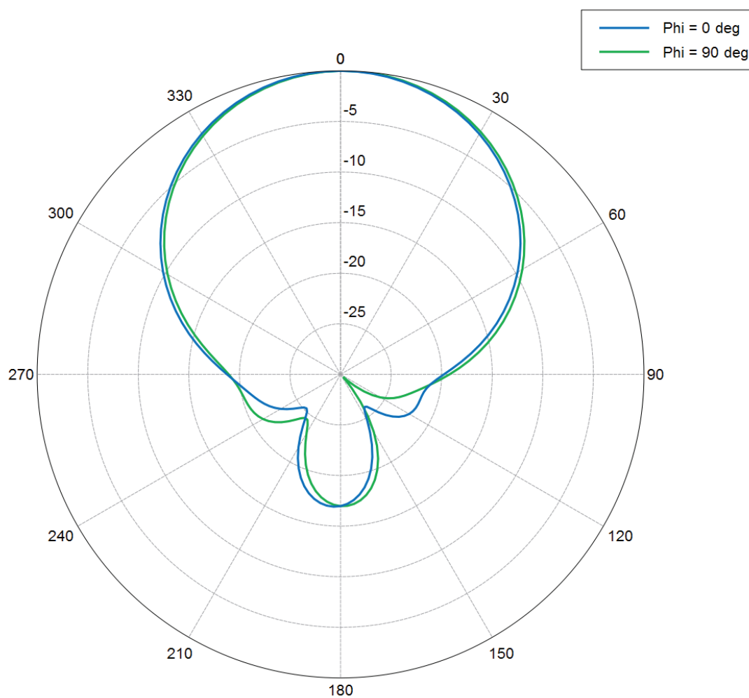
Figure 17: Antenna diagram WIRA-70-circular
