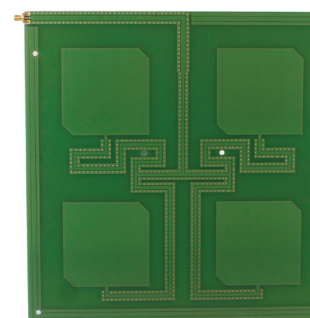
Figure 11: SSMH antenna
