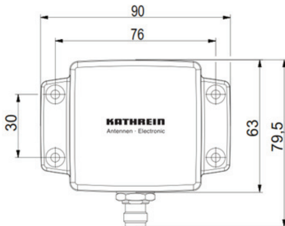
Figure 30: Dimensios for U-LORA/LORA antenna (52010092, -84, -85)
