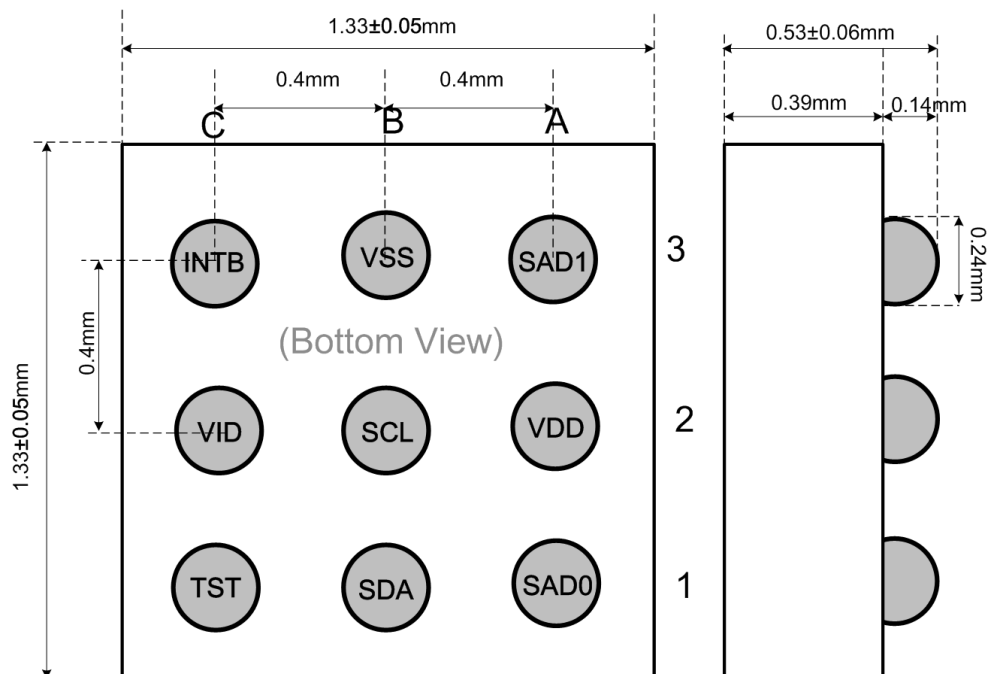
Figure 2. Package Dimensions
