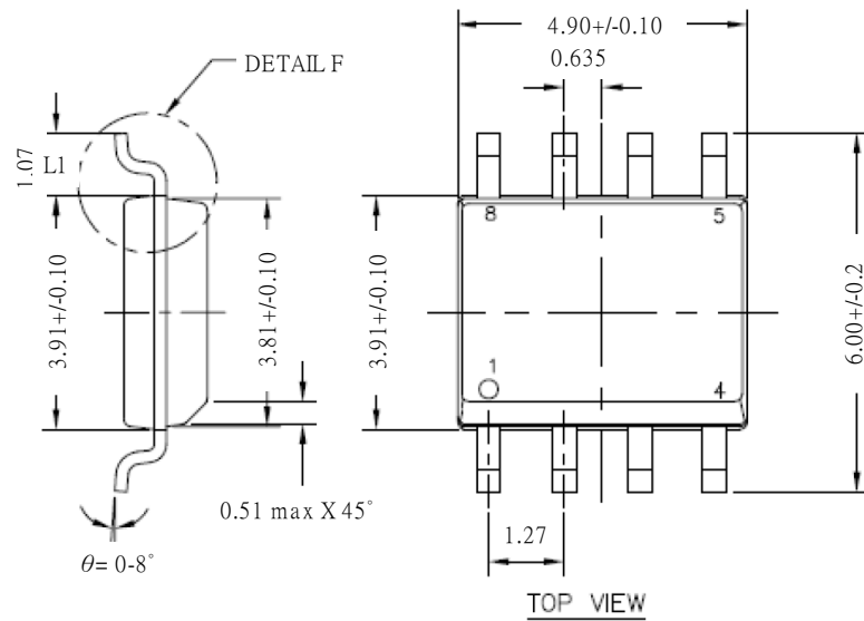
8-pin SO8-packaging
