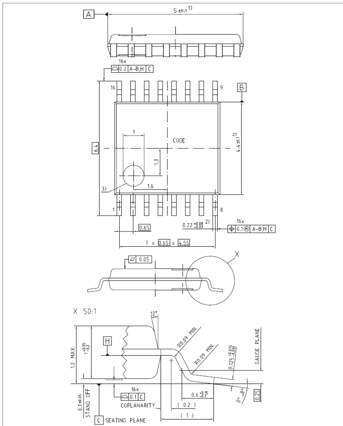
Figure 28 PG-TSSOP-16-8
