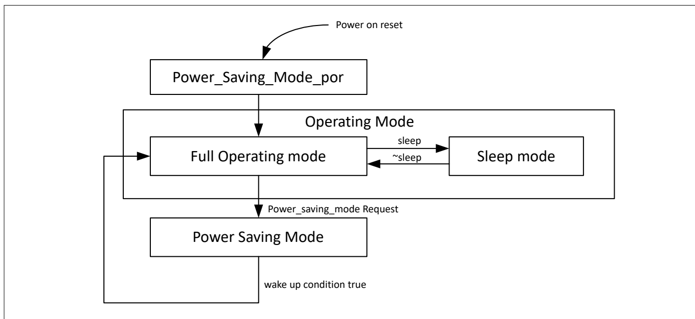
Figure 5 Power Management States
