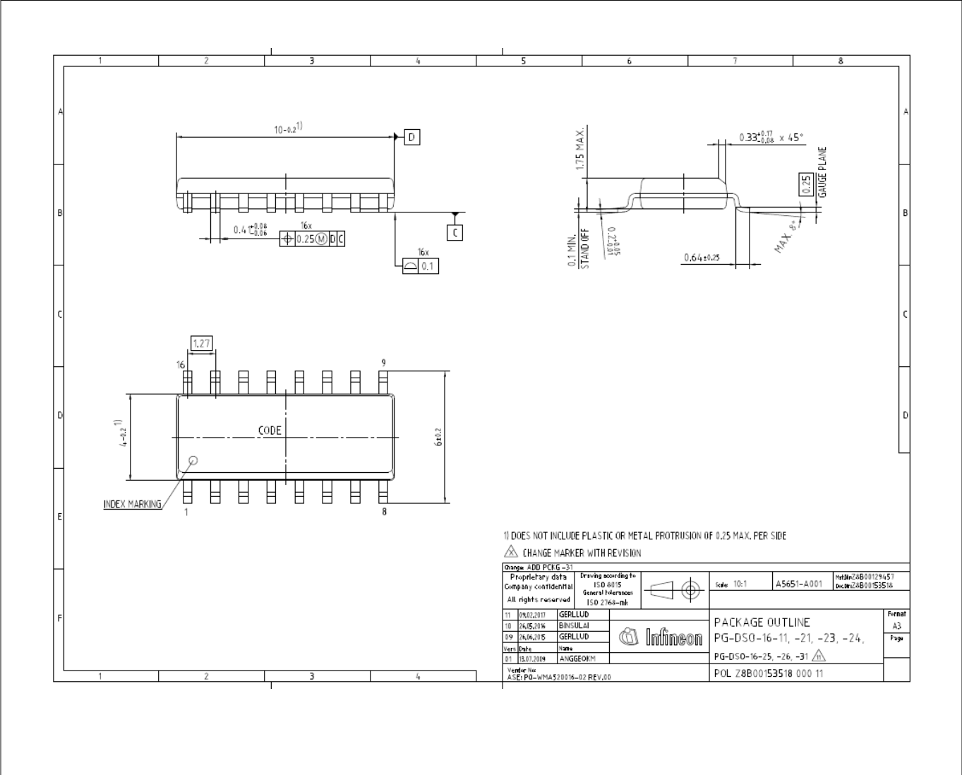
Figure 8 PG-DSO-16 Package Specification
