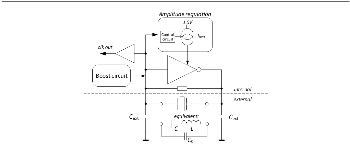
Figure 12 Pierce Oscillator
