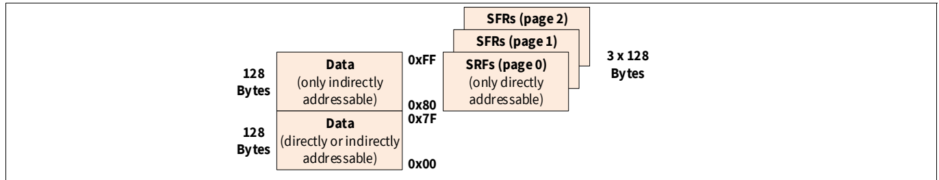
Figure 9 RAM organization
