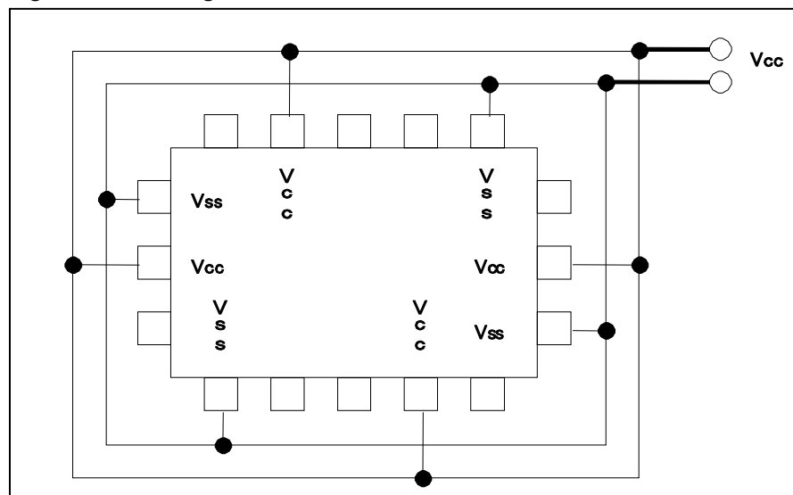
Figure 8-1 Pin Assignment
