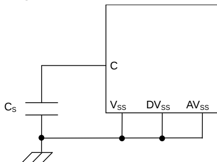
C Pin Connection Diagram
